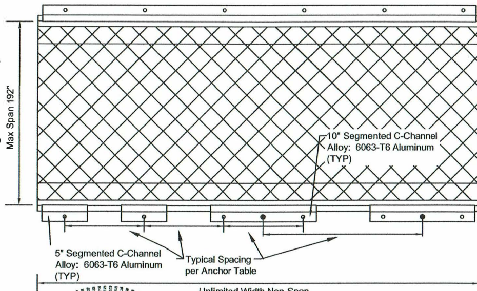
CHANNEL VERTICAL INSTALLATION (Span Sides = Welded Seam)
