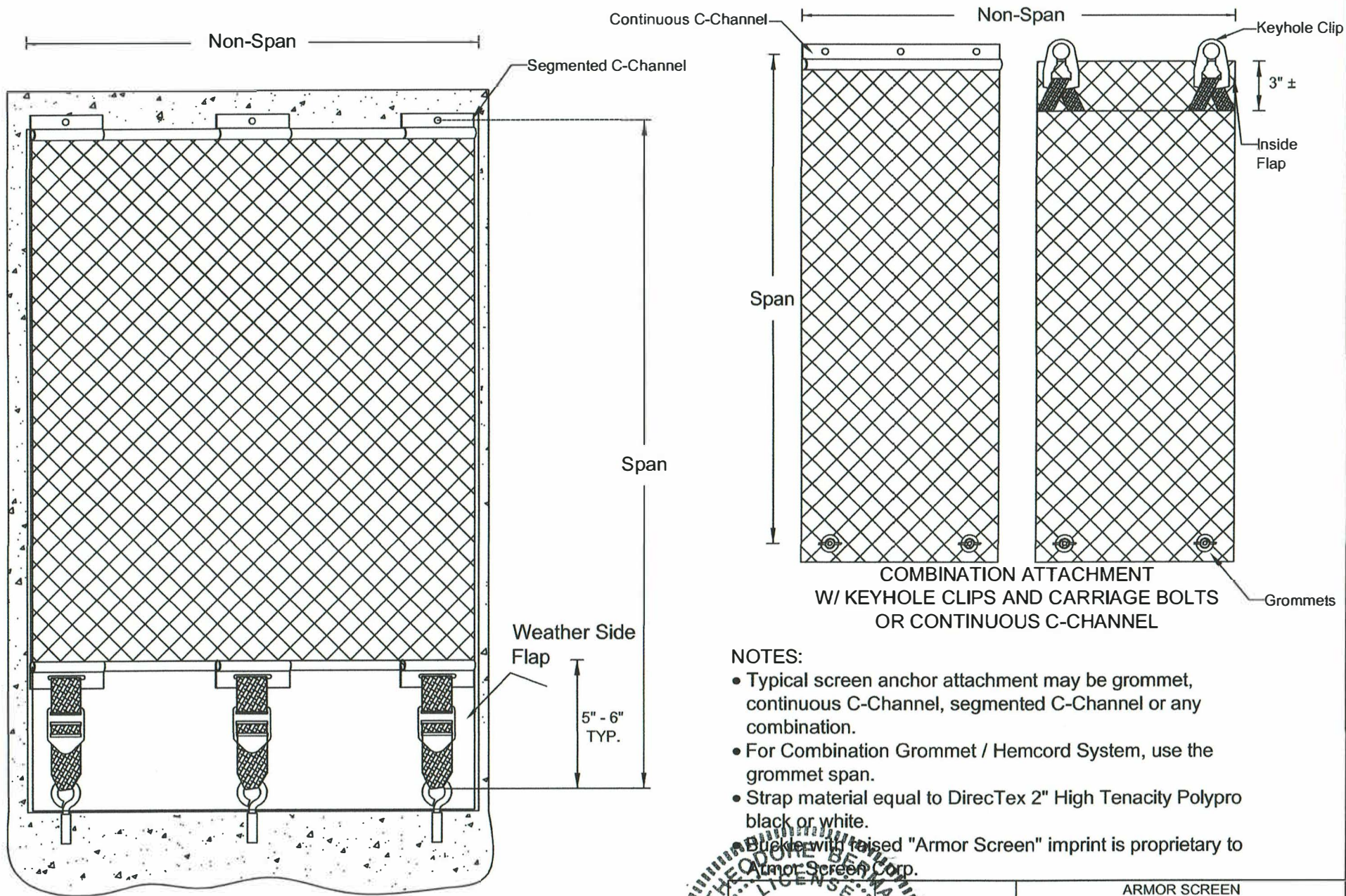
COMBINATION ATTACHMENT W/ EYEBOLT, BUCKLE/STRAP, AND SEGMENTED C-CHANNEL not to scale
