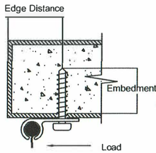
90° C-Channel
