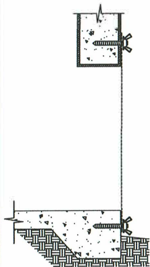
Direct Mount Typical Vertical Sectional View
