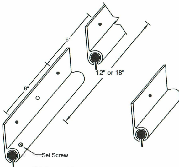
10" Segmented C-Channel Alloy: 6063-T6 Aluminum
