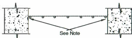
PLAN VIEW, VERTICAL SCREEN, TRAPPED OPENING
