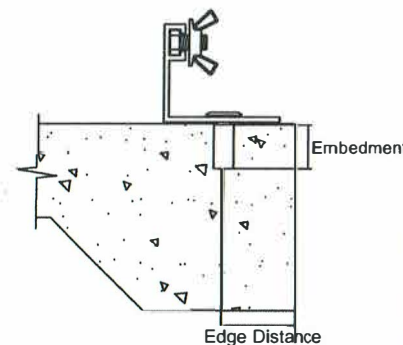
Grommet Studded / Studless Angle F-Track Minimum .125" x 6063-T6 Anchoring Detail
