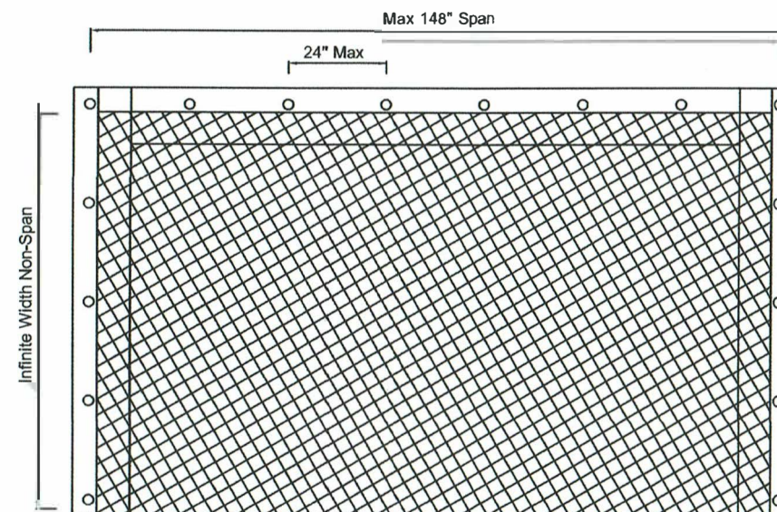
THREE SIDED SCREEN -GROMMET / C-CHANNEL
