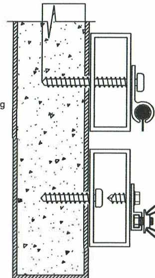
1/8" Aluminum Tube / Angle For Build-Out 6063-T6 Alloy
