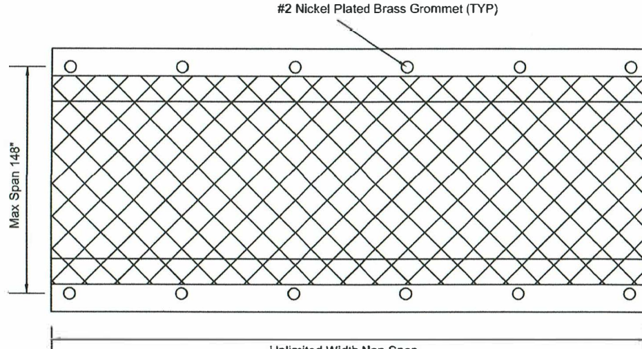
GROMMET VERTICAL INSTALLATION (Span Sides = Welded Seam)
