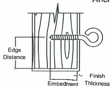
Grommet F-Track 6063-T6 (1", 2", and 3" Build-Out) Anchoring Detail
