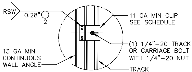
TYPICAL CLIP WELDING DETAIL
