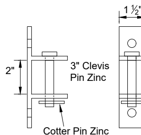
STORM BAR BRACKET Type 6063-T6
