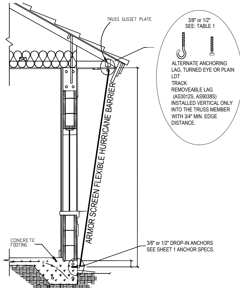
TYPICAL ONE STORY ASSEMBLY INSTALLATION
