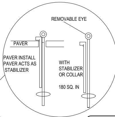
EARTH ANCHOR, 4" DIAM. HELIX HORIZONTALLY STABILIZED 24" O.C. SEE: TABLE 1
