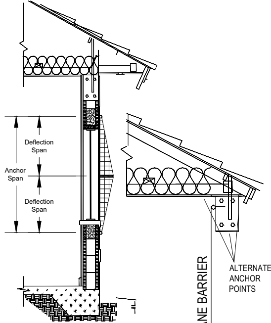
STORM BAR CONFIGURATION
