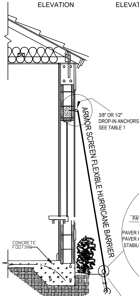
INTO EARTH ALTERNATE ASSEMBLY INSTALLATION
