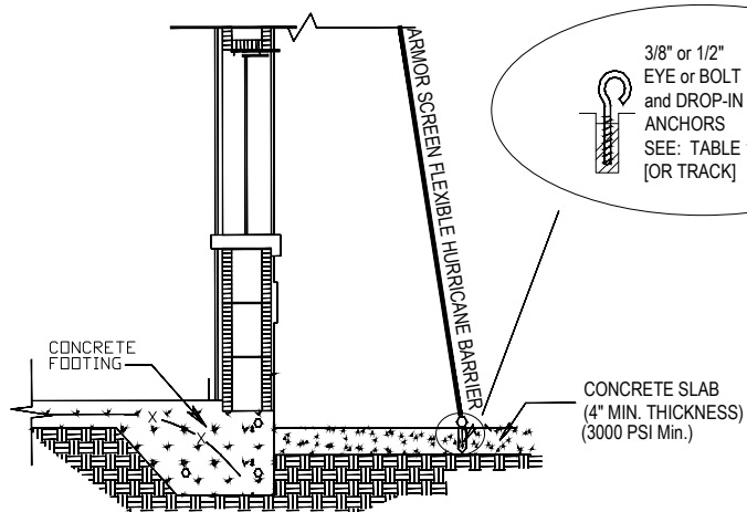
ALTERNATE ASSEMBLY INSTALLATION AT EXTERIOR SLAB
