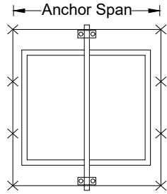
SINGE STORM BAR HORIZONTAL SCREEN ELEVATION
