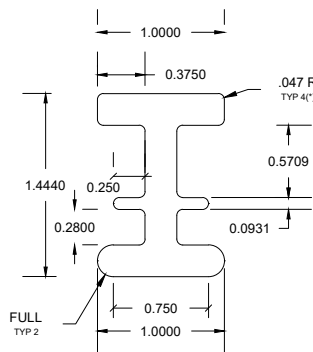
"I" TRACK ALUMINUM ALLOY 6005-T5
