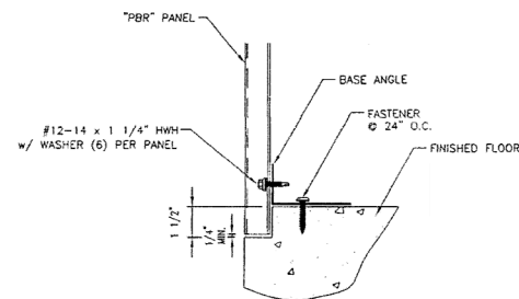
DETAIL #7 LEDGE
