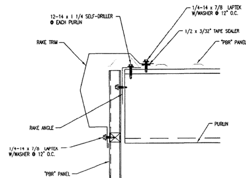
6 RAKE DETAIL SCALE : NTS
