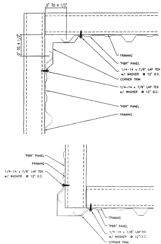
3 INSIDE/OUTSIDE CORNER DETAIL SCALE : NTS
