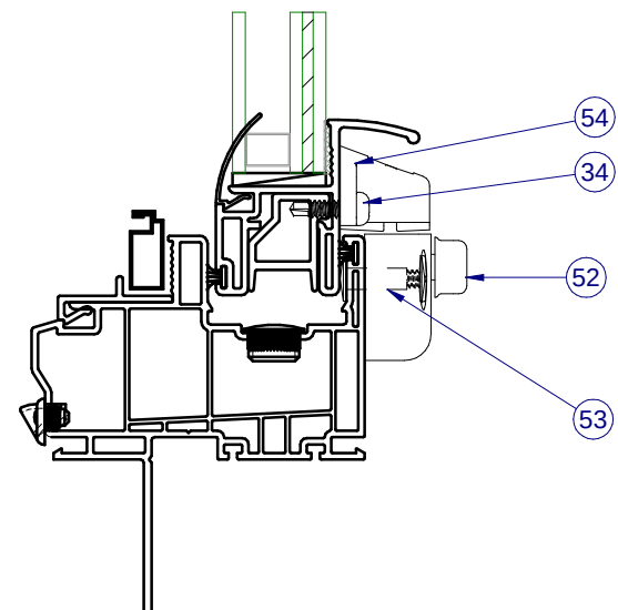
SECTION VIEW C-C ALTERNATE SWEEP LOCK SEE CHART ON PAGE 1 FOR REQUIREMENTS
