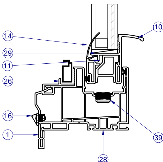
SECTION VIEW A-A NO SWEEP LOCK REQUIRED FOR WIND ZONE 3 SEE CHART ON PAGE 1 FOR REQUIREMENTS
