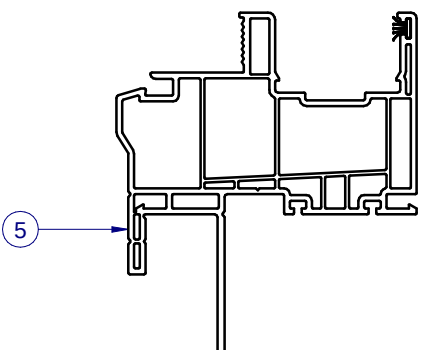
SECTION VIEW C-C ALTERNATE FIN FRAME
