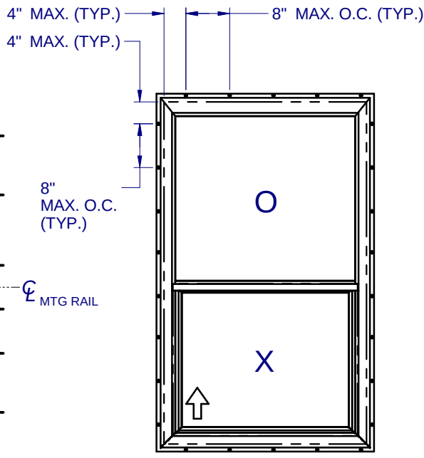
ANCHOR LAYOUT - (FIN) ALL SIZES
