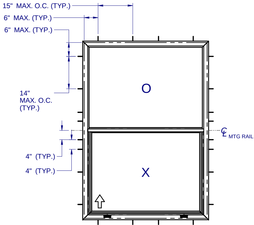
ANCHOR LAYOUT - (FLANGE) SIZES OVER 36" x 62"
