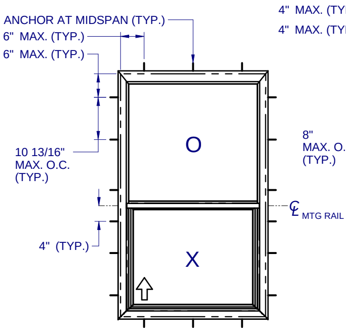
ANCHOR LAYOUT - (FLANGE) SIZES 36" x 62" AND UNDER (WINDZONE 3 W/OUT IMPACT LOCK, AND HVHZ)
