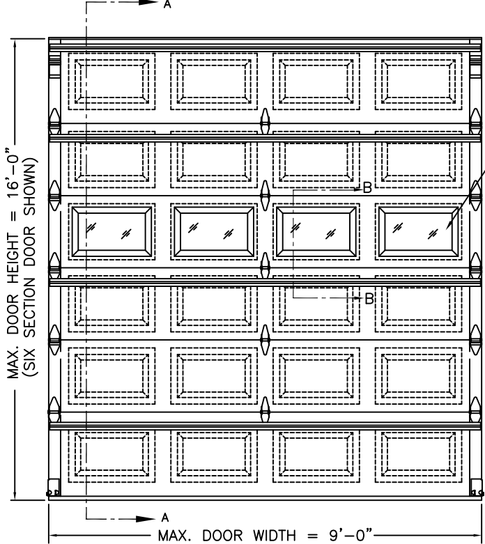
INSIDE ELEVATION
