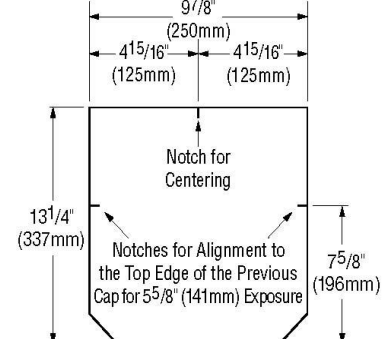
Metric Dimension
