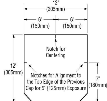
English Dimension
