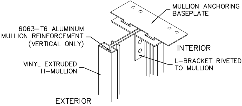
MULLION DETAIL
