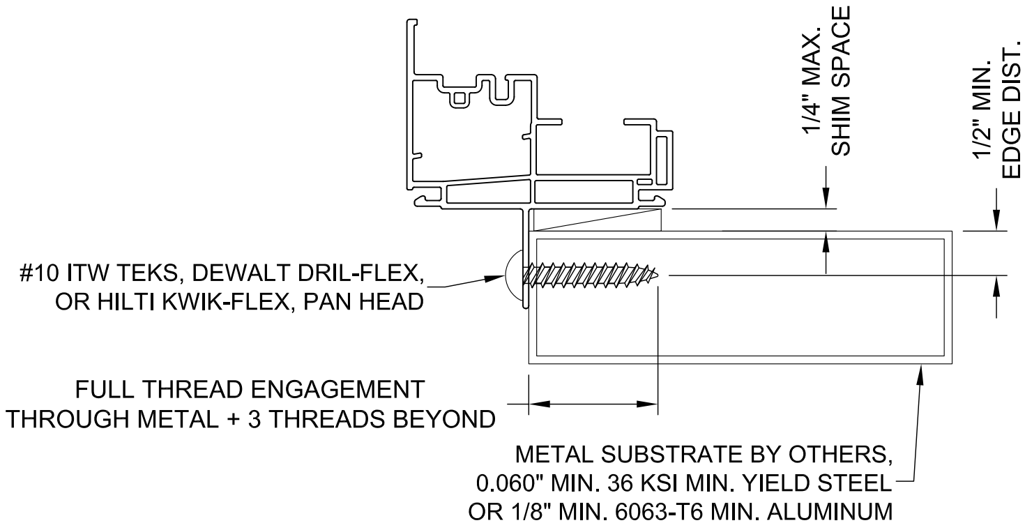
TYP. FIN METAL INSTALLATION, HEAD/JAMB (SILL SIMILAR)
