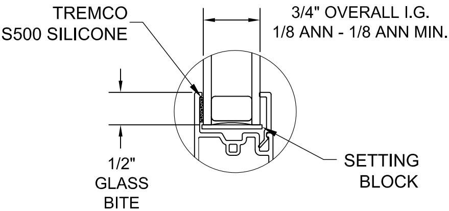
TYP. GLAZING DETAIL (FIXED SHOWN, SASH OPP.)
