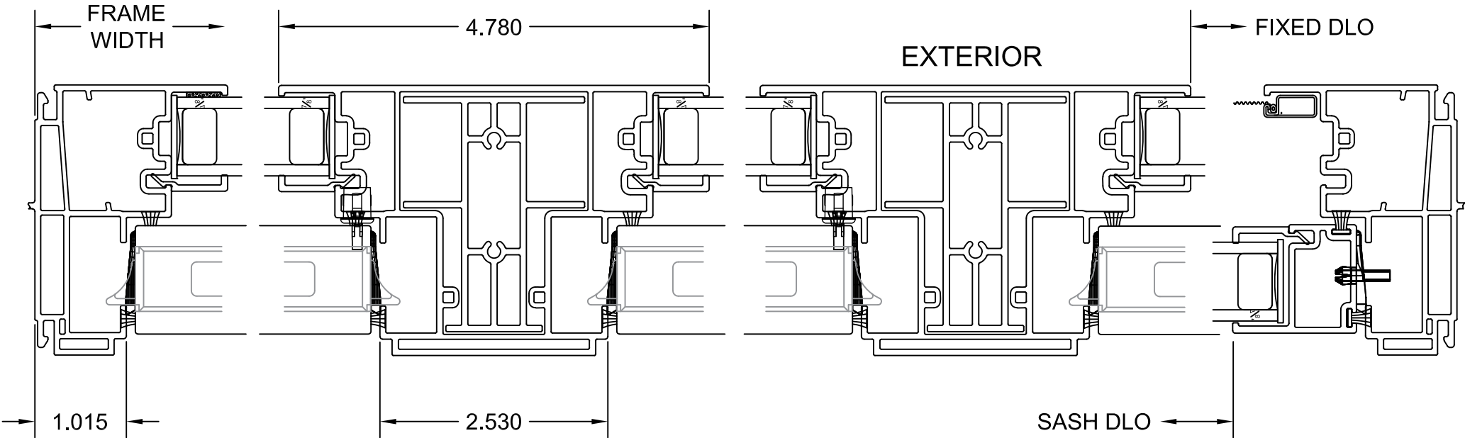
TYP. HORIZONTAL SECTION
