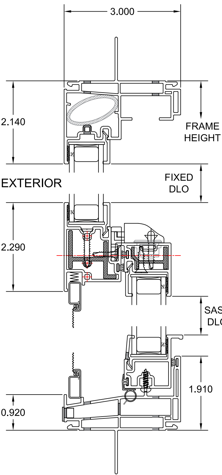
TYP. VERTICAL SECTION
