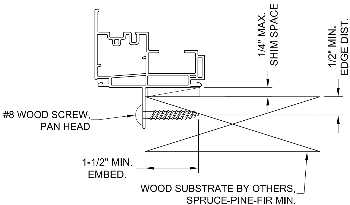
TYP. FIN WOOD INSTALLATION, HEAD/JAMB
