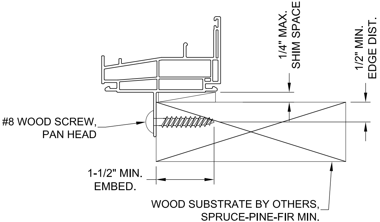
TYP. FIN WOOD INSTALLATION, SILL
