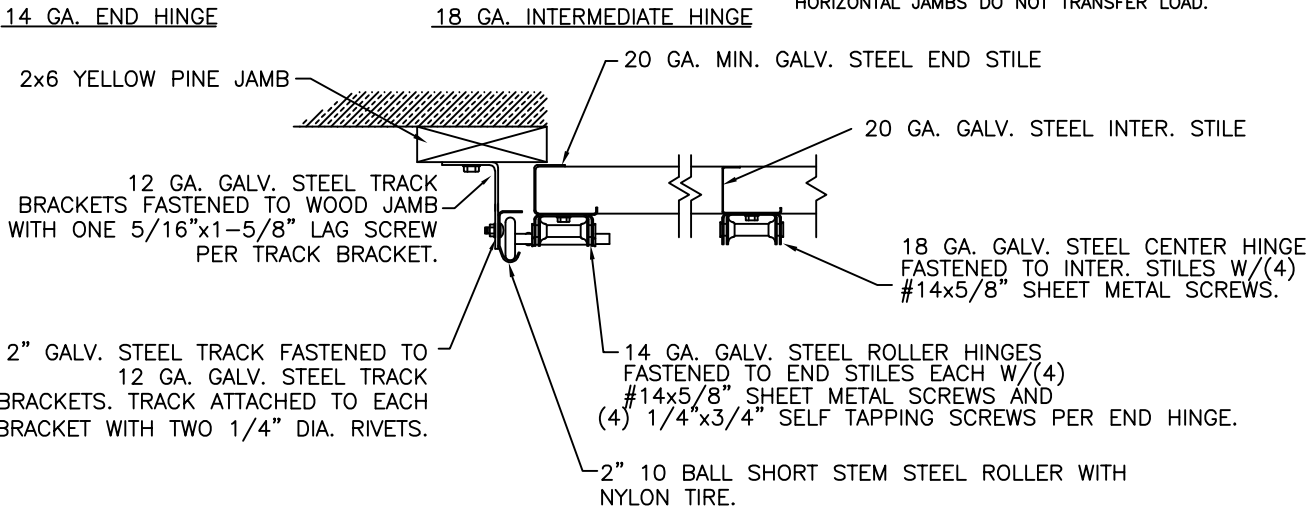
JAMB CONFIGURATION SECTION C-C
