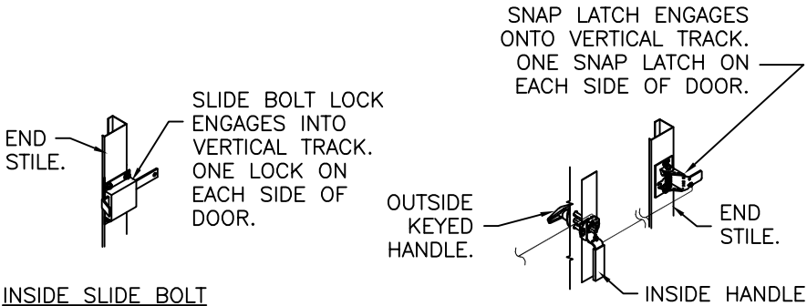
OUTSIDE KEYED LOCK WITH SNAP LATCH LOCK OPTION.
