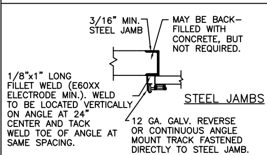
SIDE ELEVATION STANDARD-LIFT TRACK DETAILS
