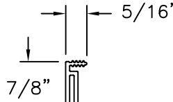
FLANGE EXTRUDED PVC
