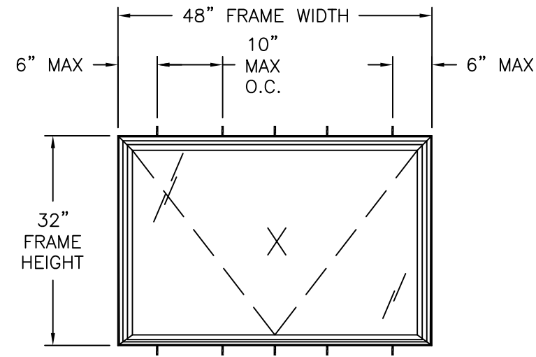
FINLESS INSTALLATION
