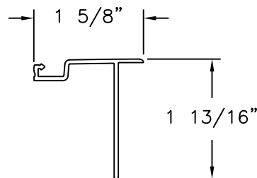
NAIL FIN & J-CHANNEL ADAPTER EXTRUDED PVC
