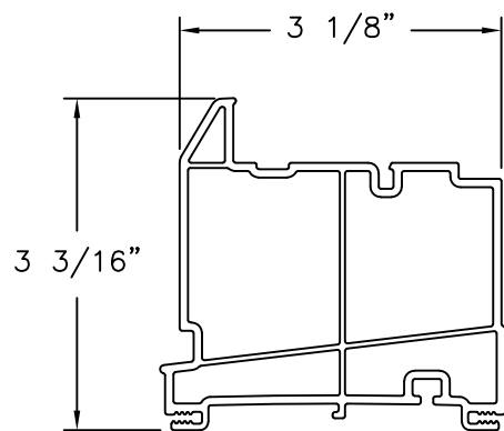
C150 HEAD EXTRUDED PVC
