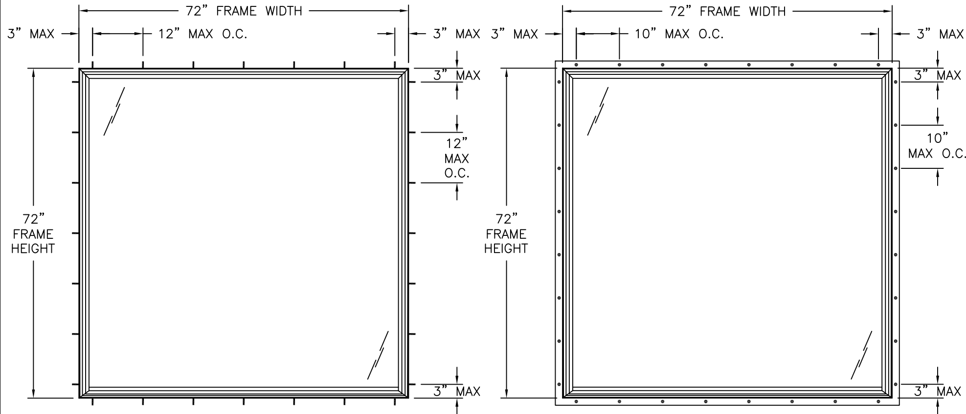
FINLESS INSTALLATION
