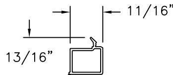
GLAZING BEAD EXTRUDED PVC
