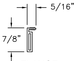
FLANGE EXTRUDED PVC
