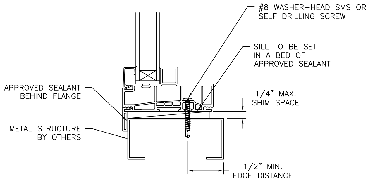
VERTICAL CROSS SECTION METAL STRUCTURE INSTALLATION
