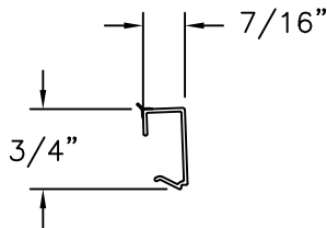
GLAZING BEAD EXTRUDED PVC
