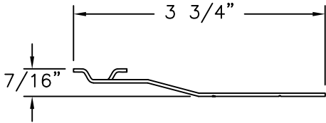
METAL CLIP GALVANIZED STEEL
