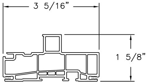
F250 SERIES HEAD EXTRUDED PVC
