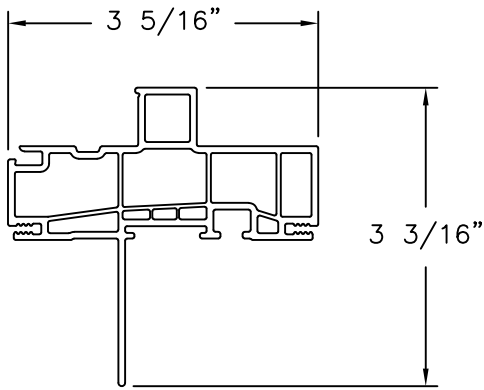
F250 SERIES HEAD WITH FIN EXTRUDED PVC
