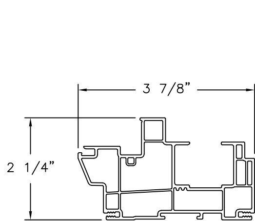
F150 HEAD EXTRUDED PVC
