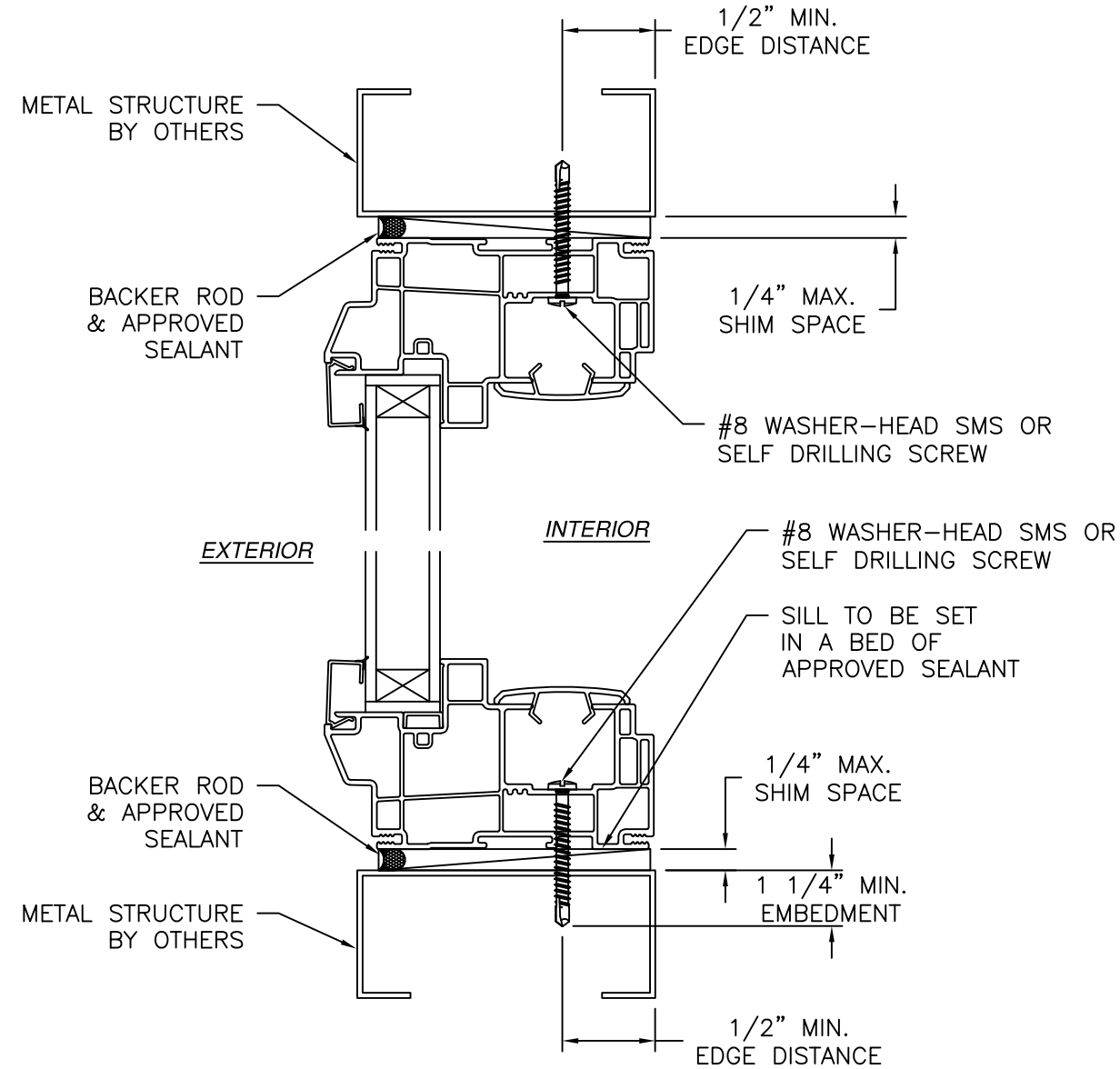
VERTICAL CROSS SECTION METAL STRUCTURE INSTALLATION
