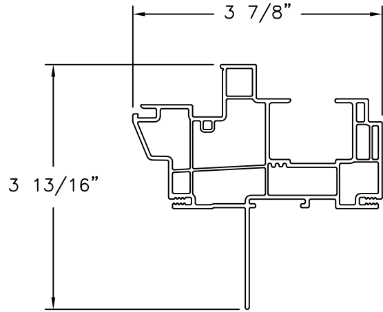
F150 HEAD WITH FIN EXTRUDED PVC
