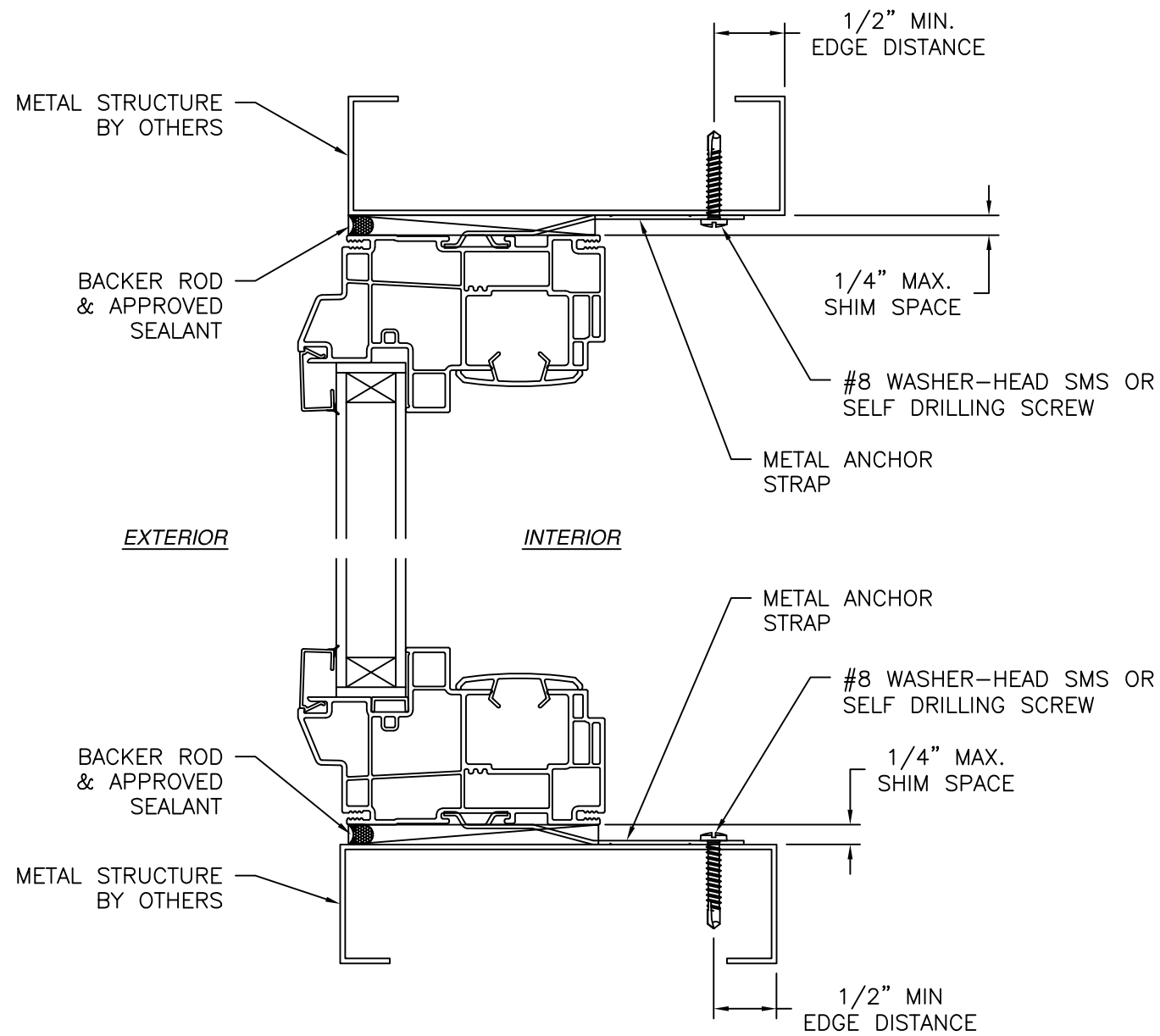
VERTICAL CROSS SECTION METAL STRUCTURE INSTALLATION
