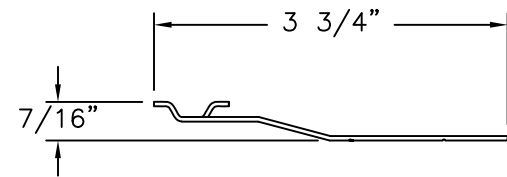
METAL CLIP GALVANIZED STEEL
