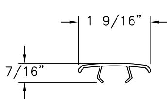
FRAME ADAPTER EXTRUDED PVC
