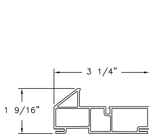
S150 HEAD EXTRUDED PVC
