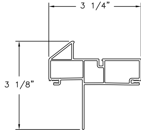
S150 HEAD WITH FIN EXTRUDED PVC
