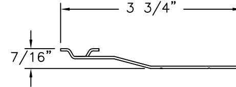
METAL CLIP GALVANIZED STEEL
