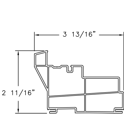
700 SERIES FRAME EXTRUDED PVC
