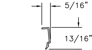
3/4" GLAZING BEAD EXTRUDED PVC
