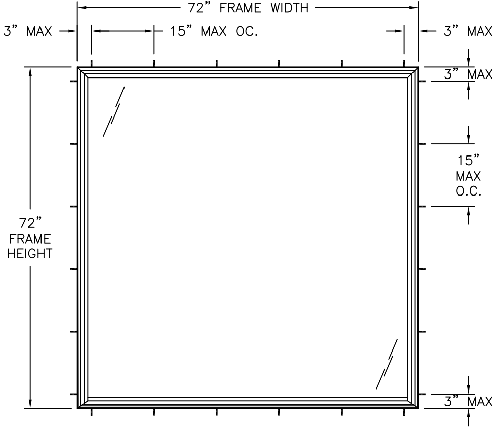
FINLESS & CLIP INSTALLATION
