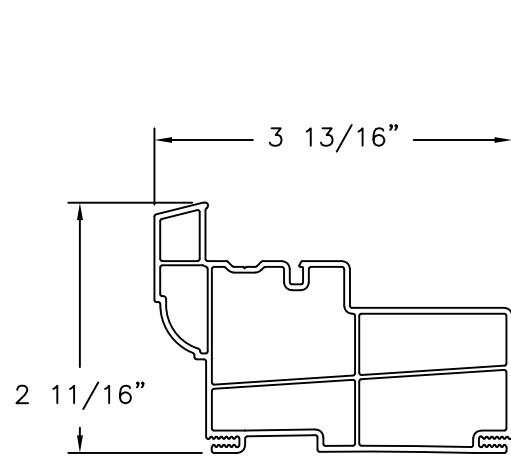
900 SERIES FRAME EXTRUDED PVC
