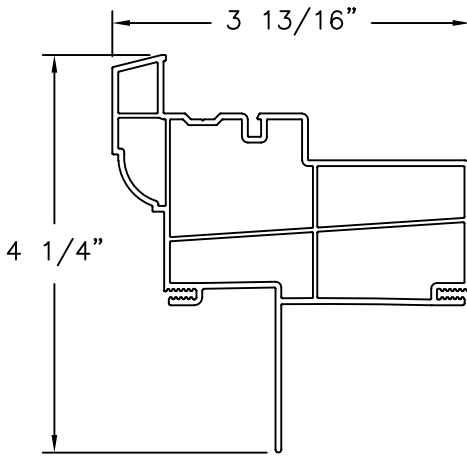
900 SERIES FRAME WITH FIN EXTRUDED PVC
