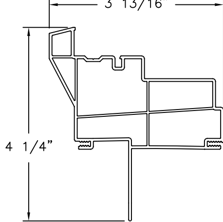
700 SERIES FRAME WITH FIN EXTRUDED PVC
