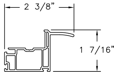
HANDLE STILE EXTRUDED PVC
