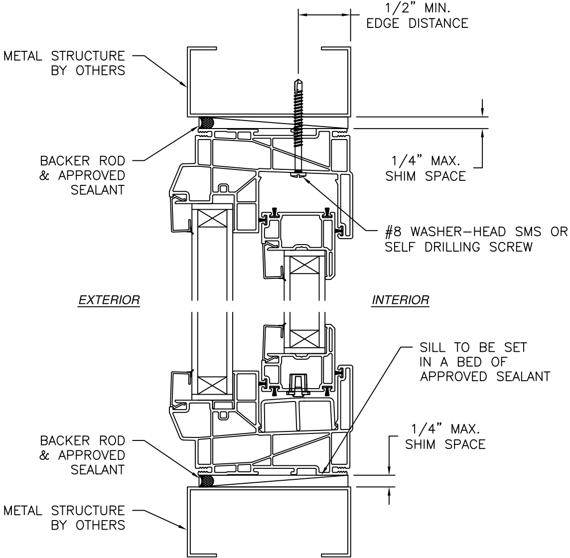
VERTICAL CROSS SECTION METAL STRUCTURE INSTALLATION
