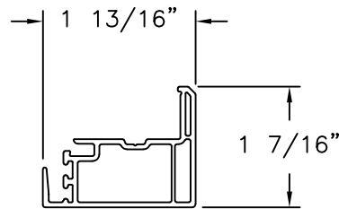
LOCK STILE EXTRUDED PVC
