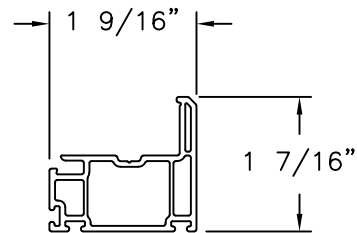
FIXED MEETING RAIL EXTRUDED PVC
