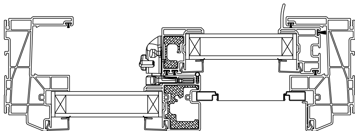
FINLESS HORIZONTAL CROSS SECTION
