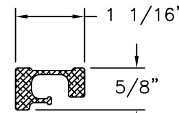
REINFORCEMENT ALUMINUM
