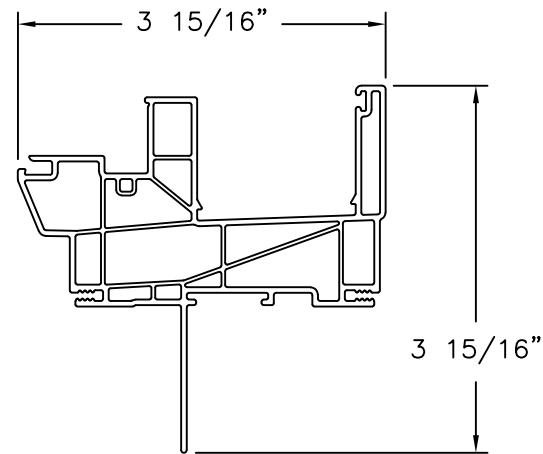
F140 SERIES HEAD WITH FIN EXTRUDED PVC
