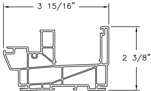
F140 SERIES HEAD EXTRUDED PVC
