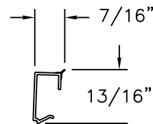
GLAZING BEAD EXTRUDED PVC
