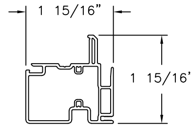
FIXED MEETING RAIL EXTRUDED PVC
