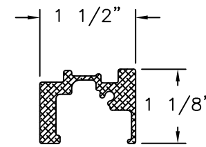
REINFORCEMENT ALUMINUM
