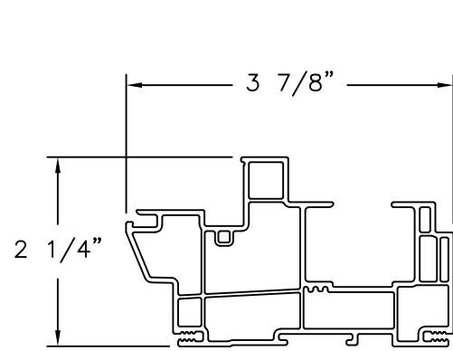
F110 SERIES HEAD EXTRUDED PVC
