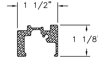
FIXED MEETING RAIL REBAR ALUMINUM
