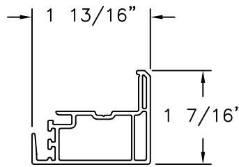
LOCK RAIL/STILE EXTRUDED PVC
