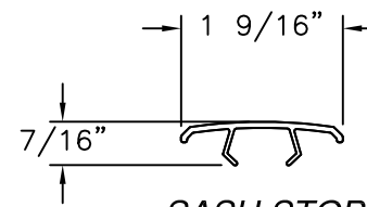
SASH STOP EXTRUDED PVC
