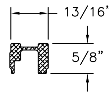
BOTTOM RAIL REINFORCEMENT ALUMINUM
