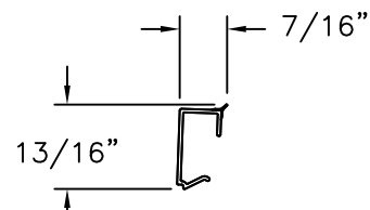
7/8" GLAZING BEAD EXTRUDED PVC
