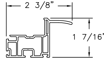
TOP RAIL EXTRUDED PVC
