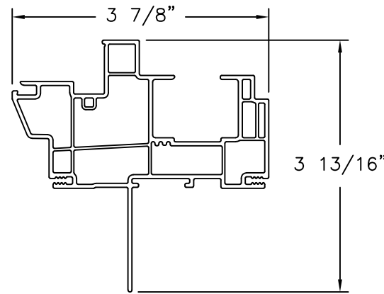
F110 SERIES JAMB WITH FIN EXTRUDED PVC
