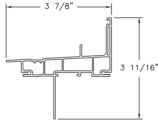
F110 SERIES SILL WITH FIN EXTRUDED PVC
