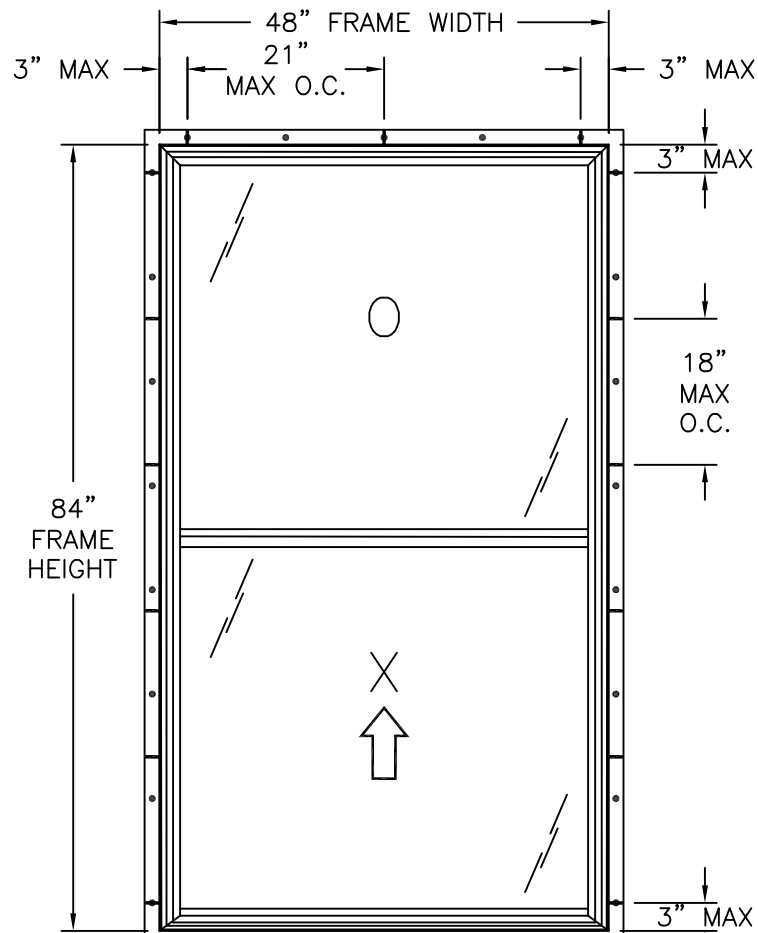
FINLESS & CLIP INSTALLATION
