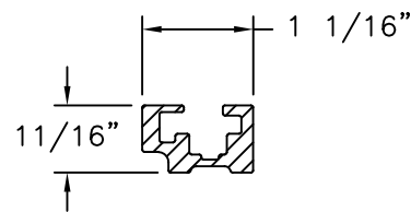
SASH INTERLOCK REINFORCEMENT ALUMINUM
