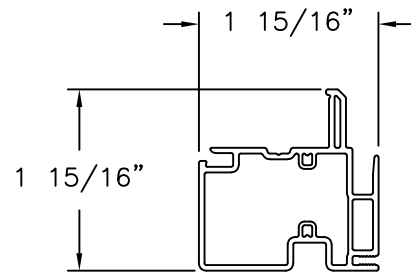
FIXED MEETING RAIL/STILE EXTRUDED PVC
