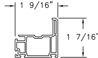
STILE EXTRUDED PVC
