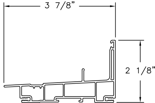
F110 SERIES SILL EXTRUDED PVC
