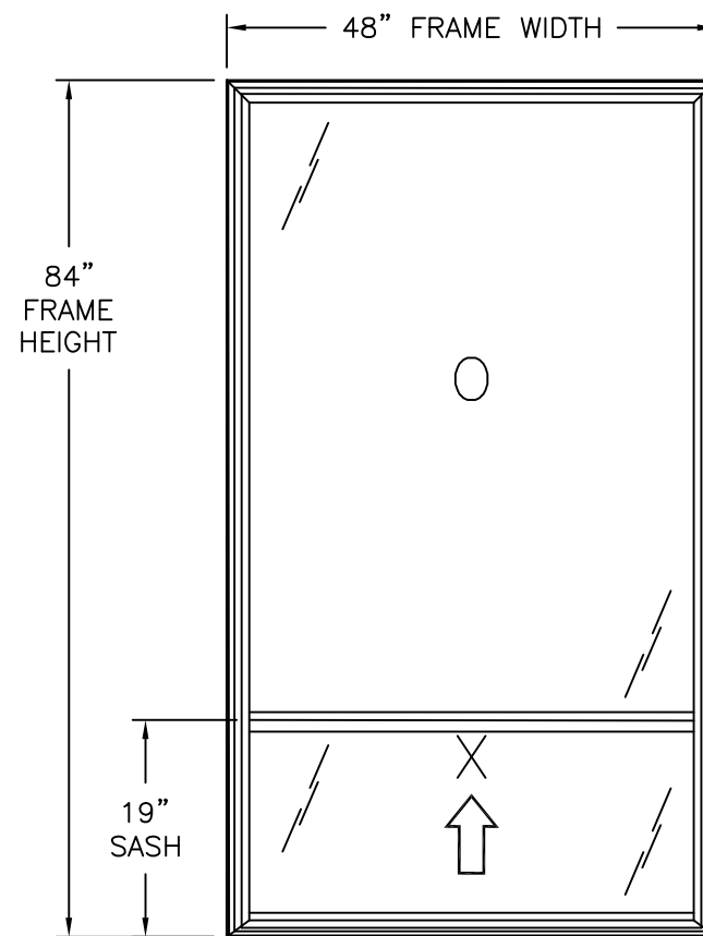
ORIEL CONFIGURATION ANCHORING SIMILAR TO EQUAL LEG UNIT
