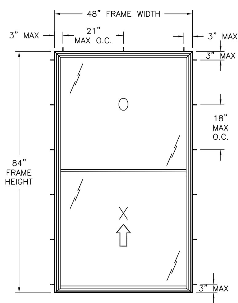
FINLESS & CLIP INSTALLATION
