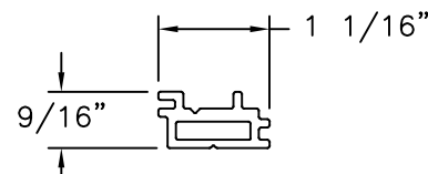
REINFORCEMENT ALUMINUM
