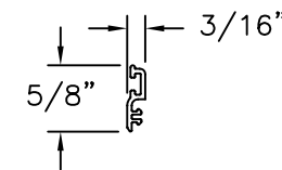
SILL RISER EXTRUDED PVC
