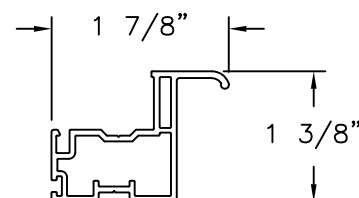
BOTTOM LIFT RAIL EXTRUDED PVC
