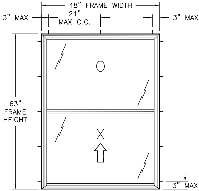
FINLESS & CLIP INSTALLATION
