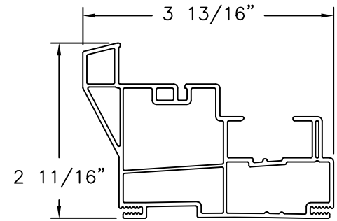
700 SERIES JAMB EXTRUDED PVC
