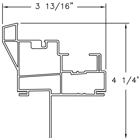
700 SERIES JAMB WITH FIN EXTRUDED PVC
