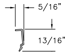
3/4" GLAZING BEAD EXTRUDED PVC
