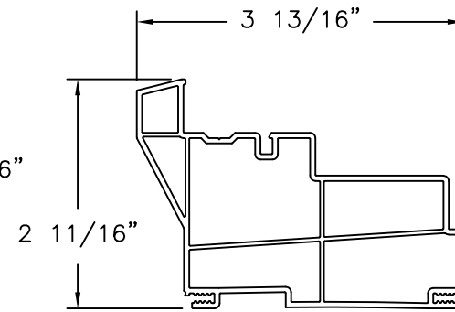
700 SERIES HEAD EXTRUDED PVC
