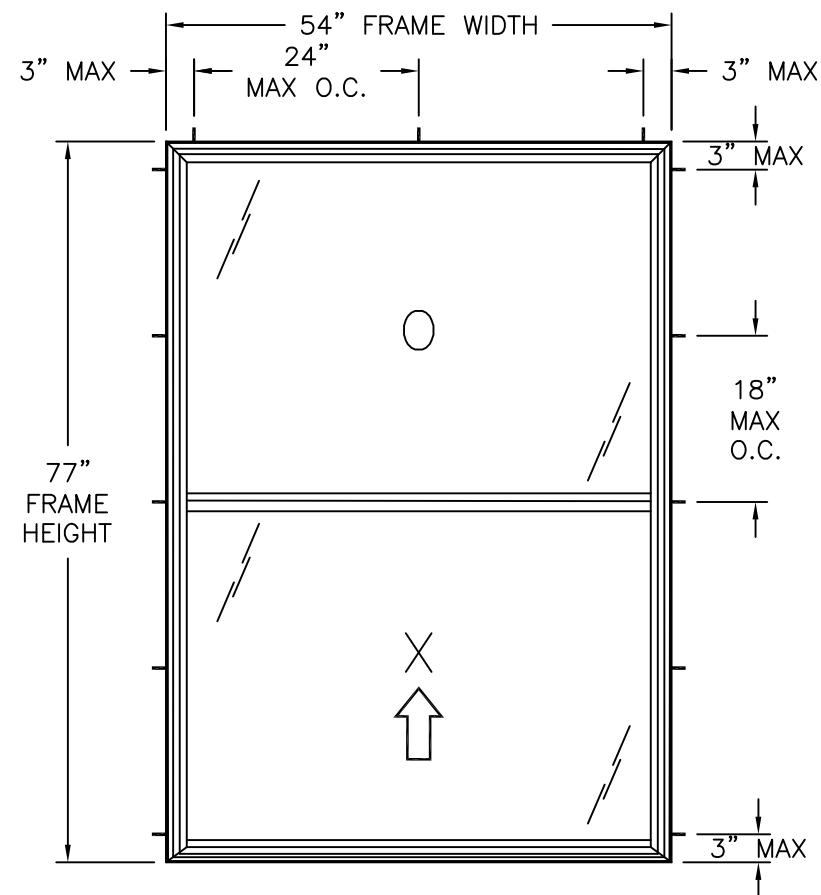
FINLESS & CLIP INSTALLATION
