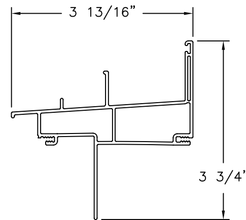
900 SERIES SILL WITH FIN EXTRUDED PVC
