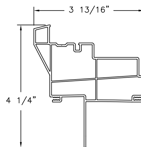
700 SERIES HEAD WITH FIN EXTRUDED PVC
