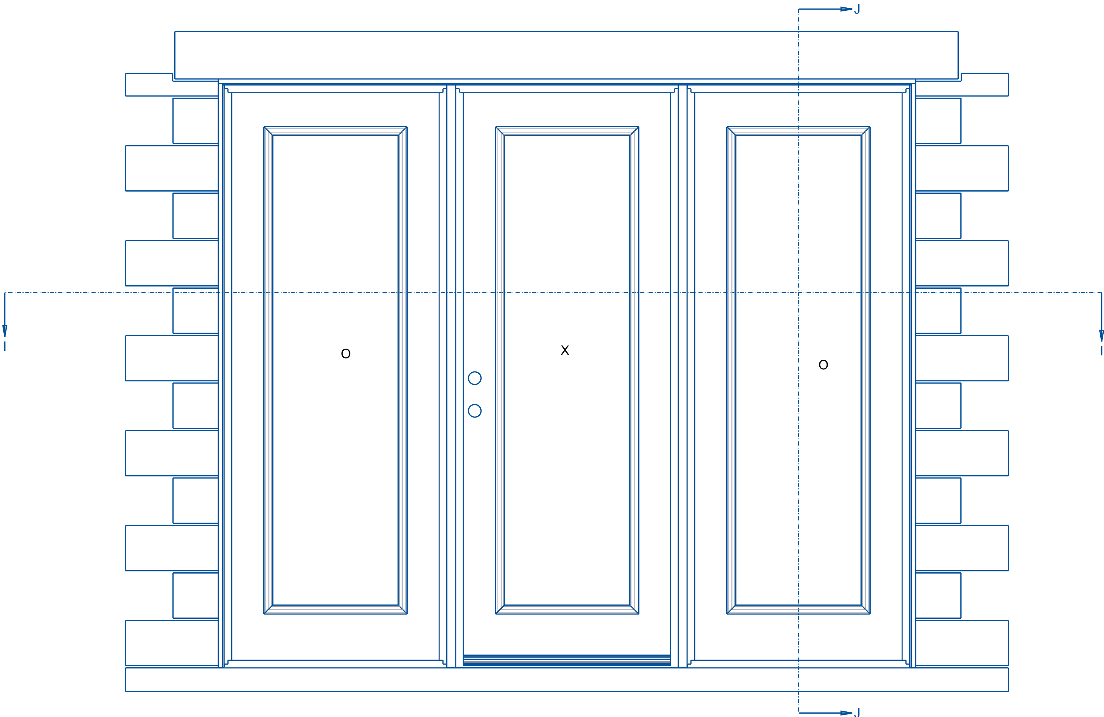
SINGLE DOOR WITH SIDELITES (OXO) INSTALLATION INSWING SHOWN
