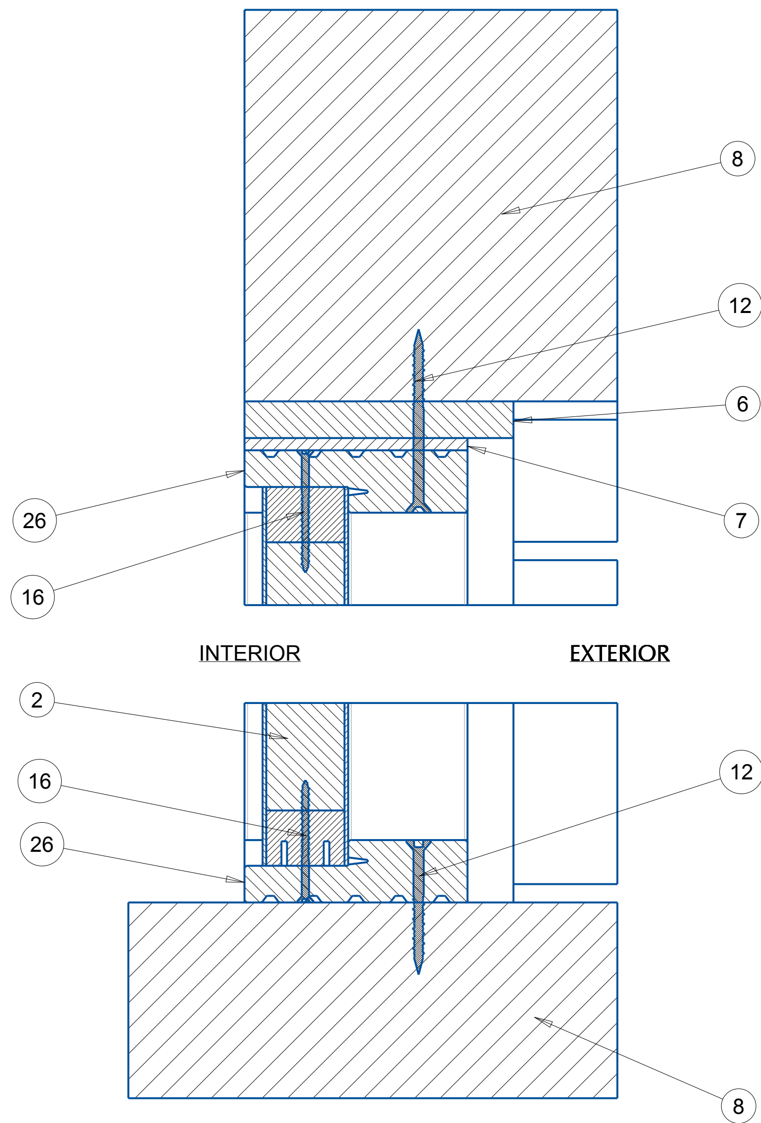
SECTION J-J
