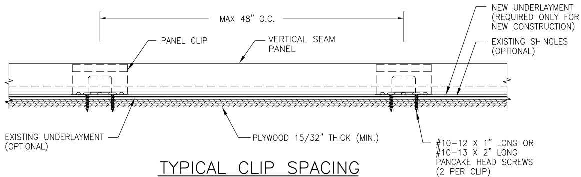
DETAIL 1
