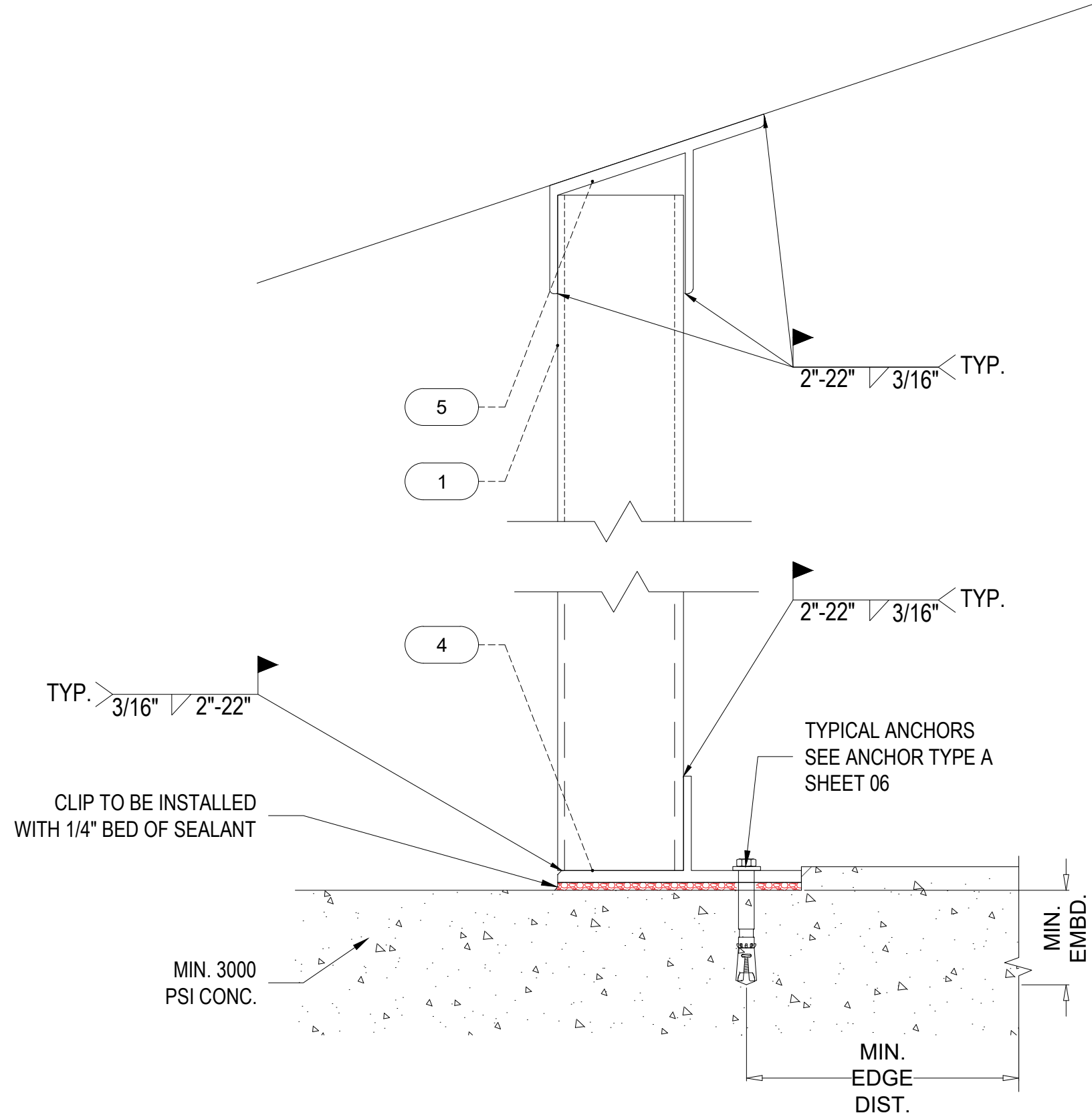
S1 TOP CONNECTION DETAIL
