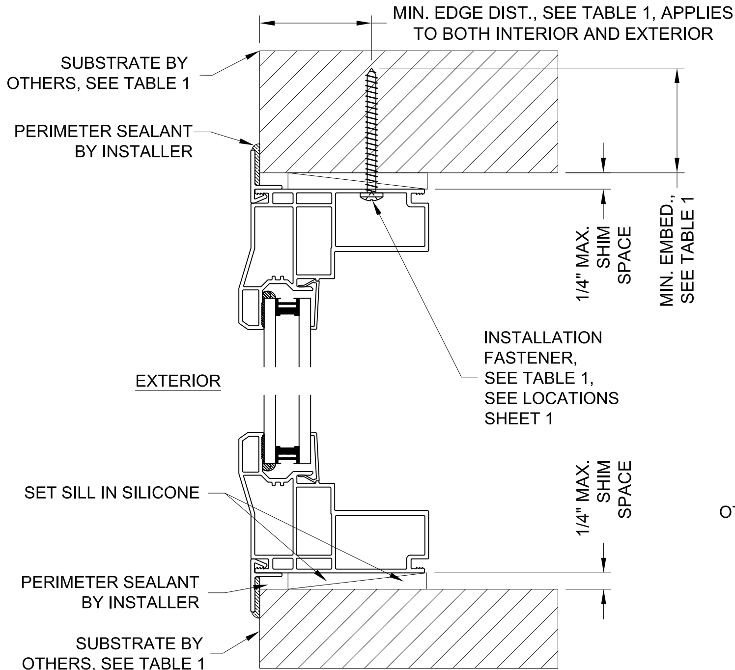
TYPICAL FRAME VERTICAL SECTION
