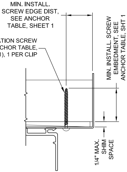
OPTIONAL INSTALLATION SCREW THROUGH CLIP
