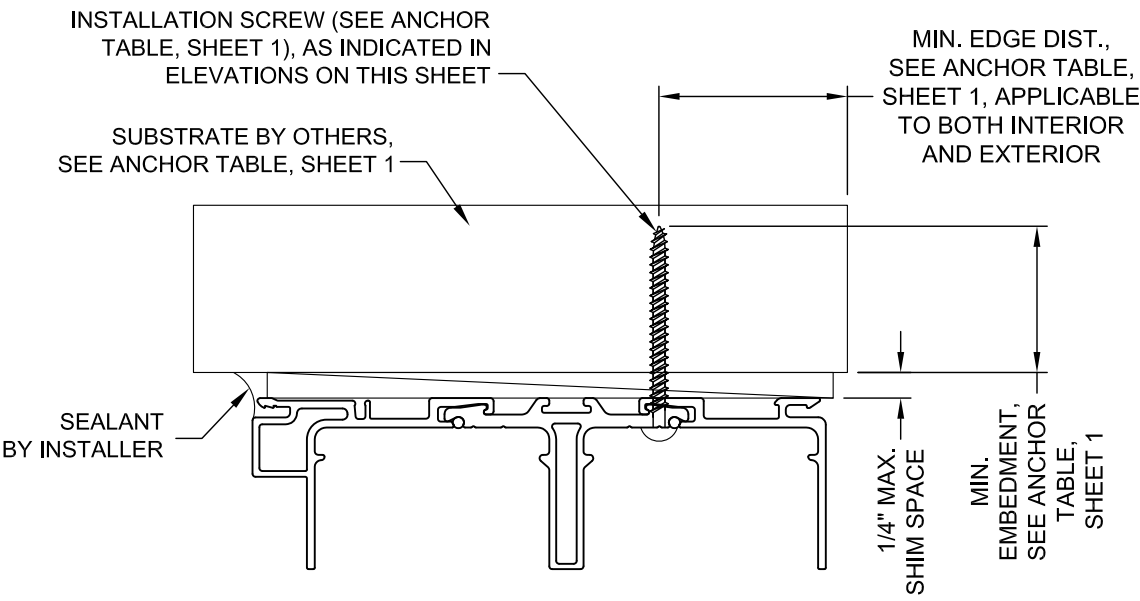
TYP. HEAD/JAMB SCREW INSTALLATION
