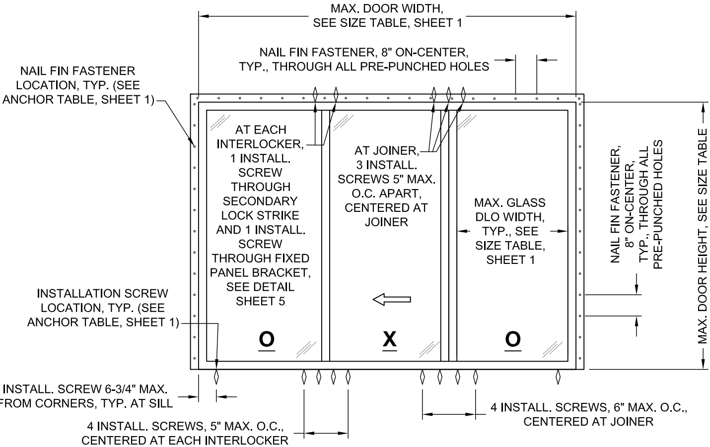
TYP. OXO OR OXXO FIN INSTALLATION
