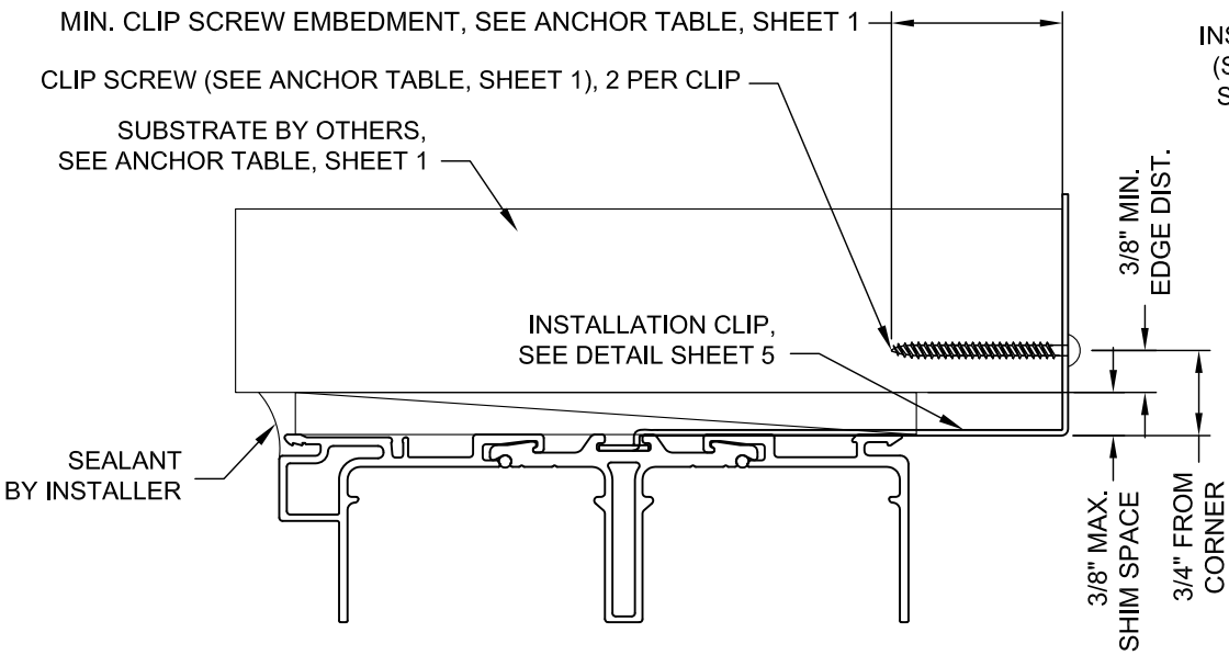
TYP. HEAD/JAMB CLIP INSTALLATION
