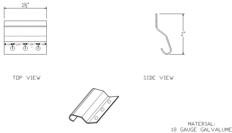
Figure 1 – MIP Series Clip
