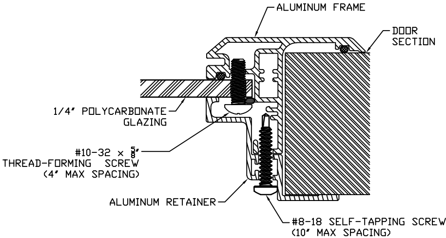
IMPACT-RESISTANT ASSEMBLY DETAILS DRAWING 105042-A
