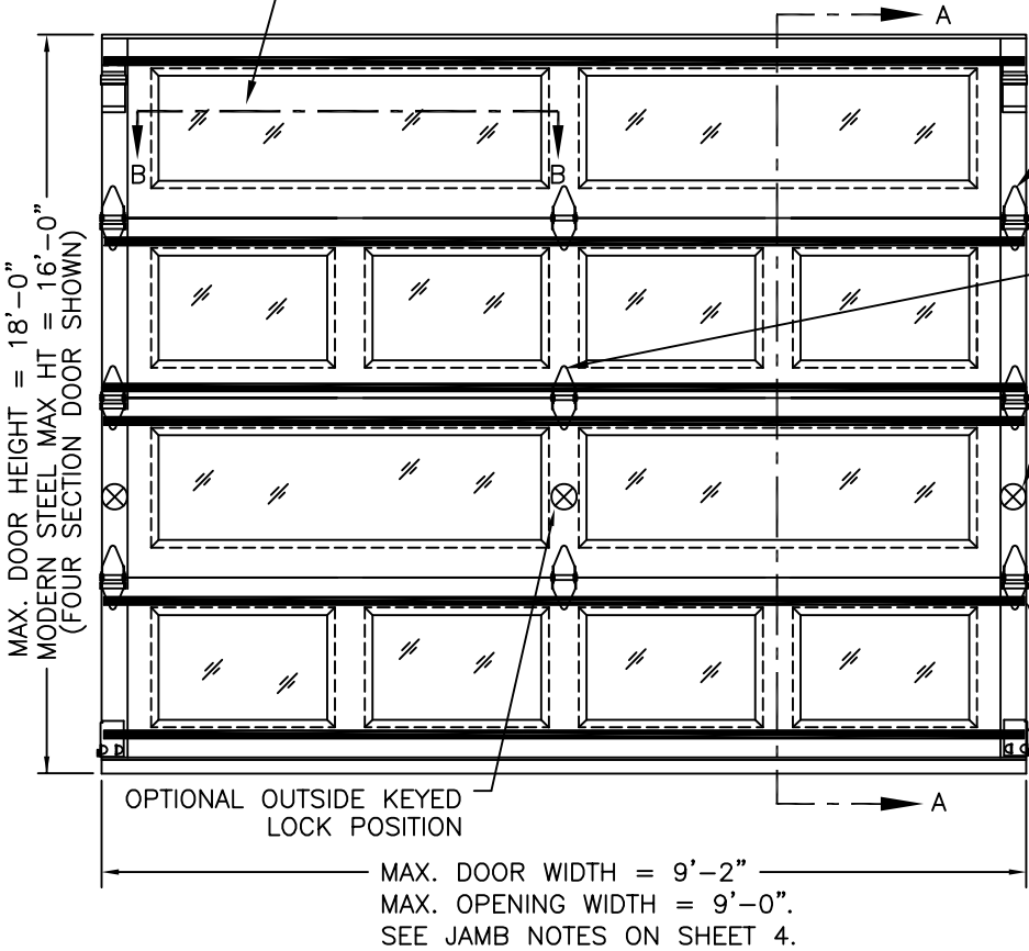
REPRESENTATIVE GLAZING PATTERNS.
