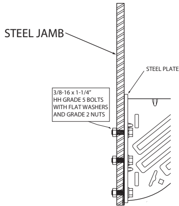
BRACKET MOUNTING TO STEEL DETAIL
