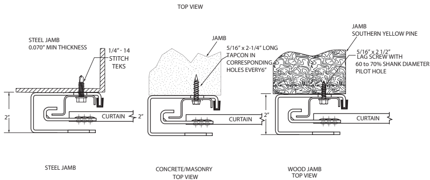
GUIDE MOUNT DETAIL
