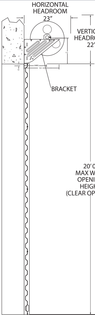
SIDE VIEW
