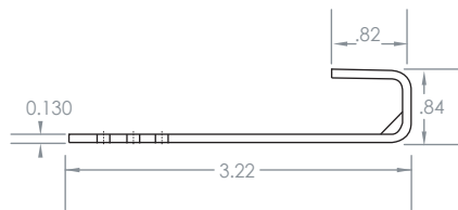
WINDCLIP
