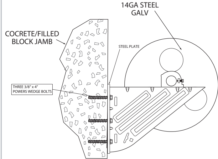
BRACKET MOUNTING TO MASONRY DETAIL
