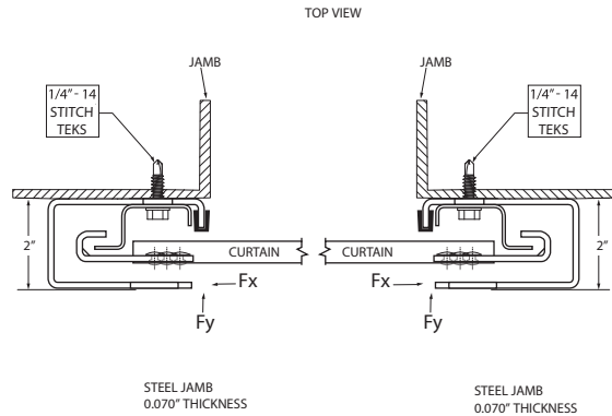
RIGHT AND LEFT GUIDE MOUNT DETAIL LOAD DIAGRAM MIN 0.070" STEEL JAM SHOWN
