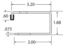
GUIDE DETAIL 14GA STEEL
