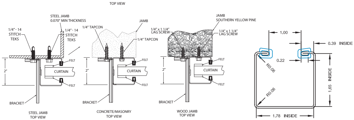
GUIDE MOUNT DETAIL
