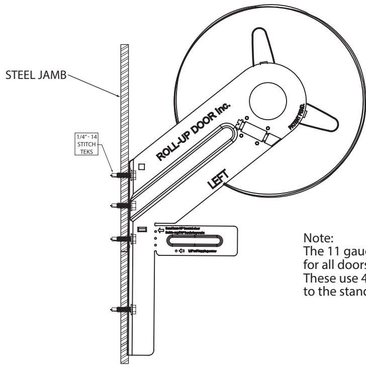
EXTENDED BRACKET MOUNTING TO STEEL DETAIL
