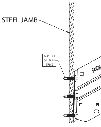
BRACKET MOUNTING TO STEEL DETAIL
