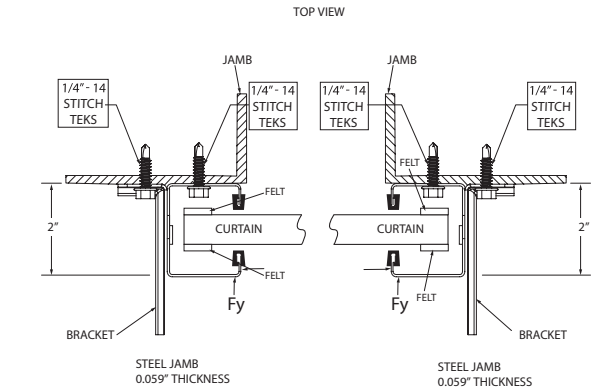
RIGHT AND LEFT GUIDE MOUNT DETAIL LOAD DIAGRAM MIN 0.070\"/>
