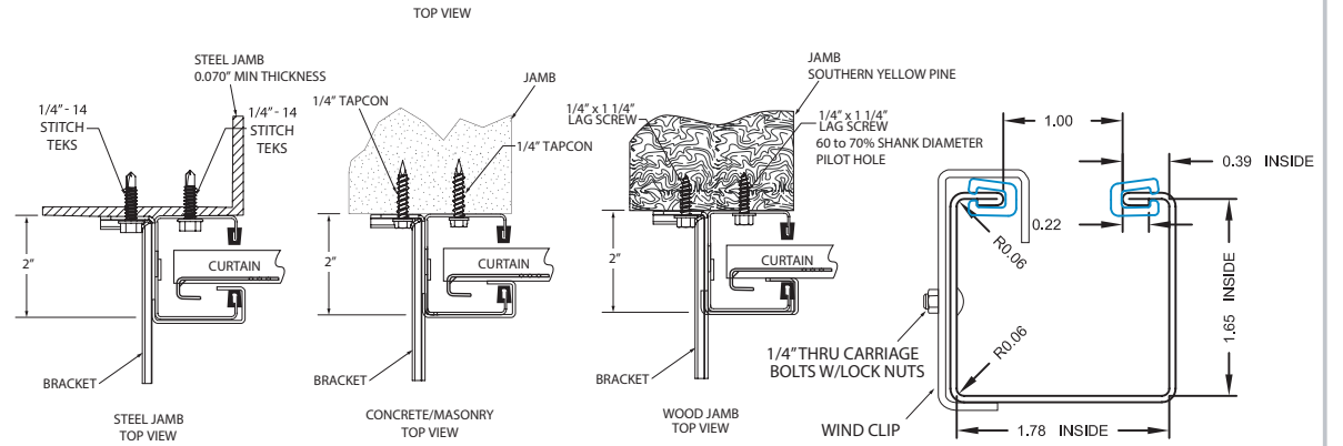
GUIDE DETAIL 18GA STEEL
