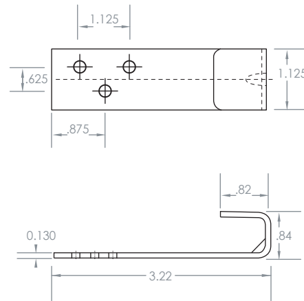
WIND CLIP DETAIL
