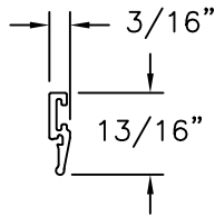
GLASS BEAD ALUMINUM 6063-T6
