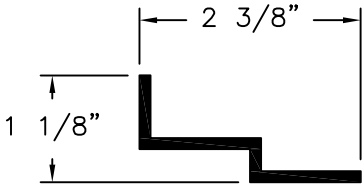
L BRACKET ALUMINUM 6063-T5
