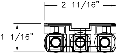
TOP AND BOTTOM BEARING SET STAINLESS STEEL
