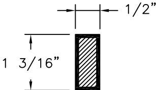
TWIN CORE ALUMINUM 6063-T5
