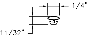
O SHAPE GASKET RUBBER
