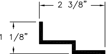
L BRACKET ALUMINUM 6063-T5
