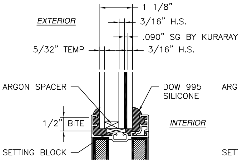
GLAZING DETAIL A
