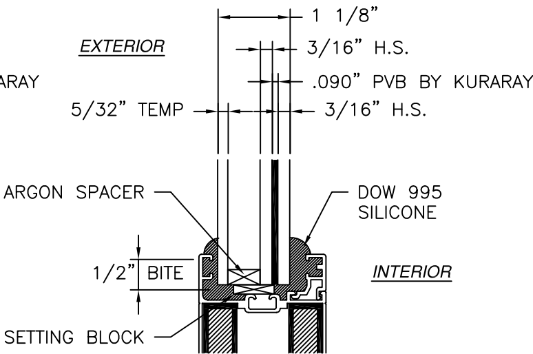
GLAZING DETAIL B
