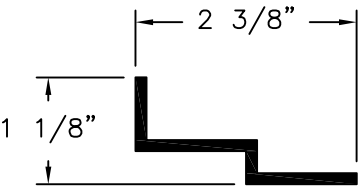
L BRACKET ALUMINUM 6063-T5
