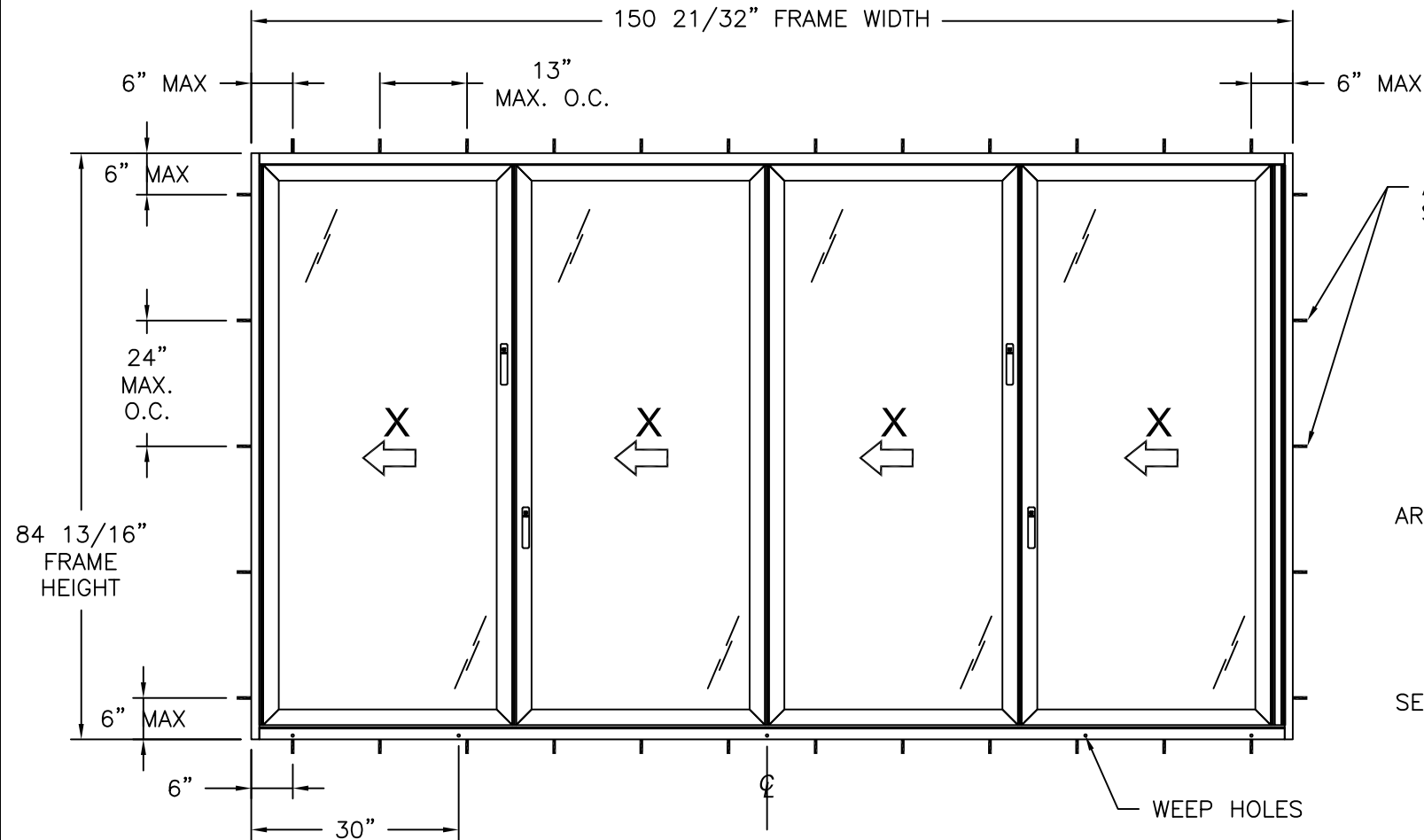
FD54 TWIN CORE ALUMINUM BIFOLD DOOR INTERIOR VIEW
