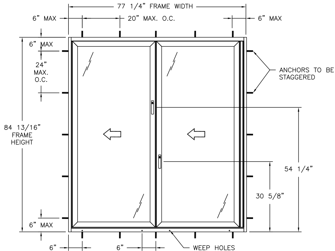
FD54 TWIN CORE ALUMINUM BIFOLD DOOR INTERIOR VIEW
