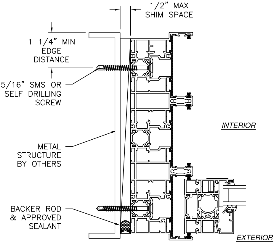
JAMB INSTALLATION DETAIL METAL STRUCTURE INSTALLATION 3-TRACK SYSTEM SHOWN, 2-TRACK SYSTEM SIMILAR
