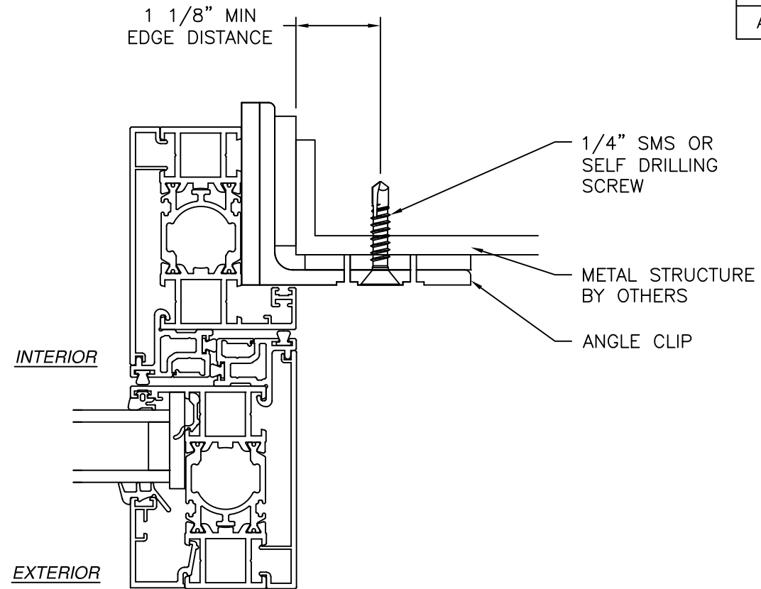
POCKET JAMB INSTALLATION DETAIL
