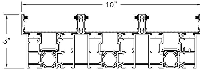
3-TRACK FRAME
