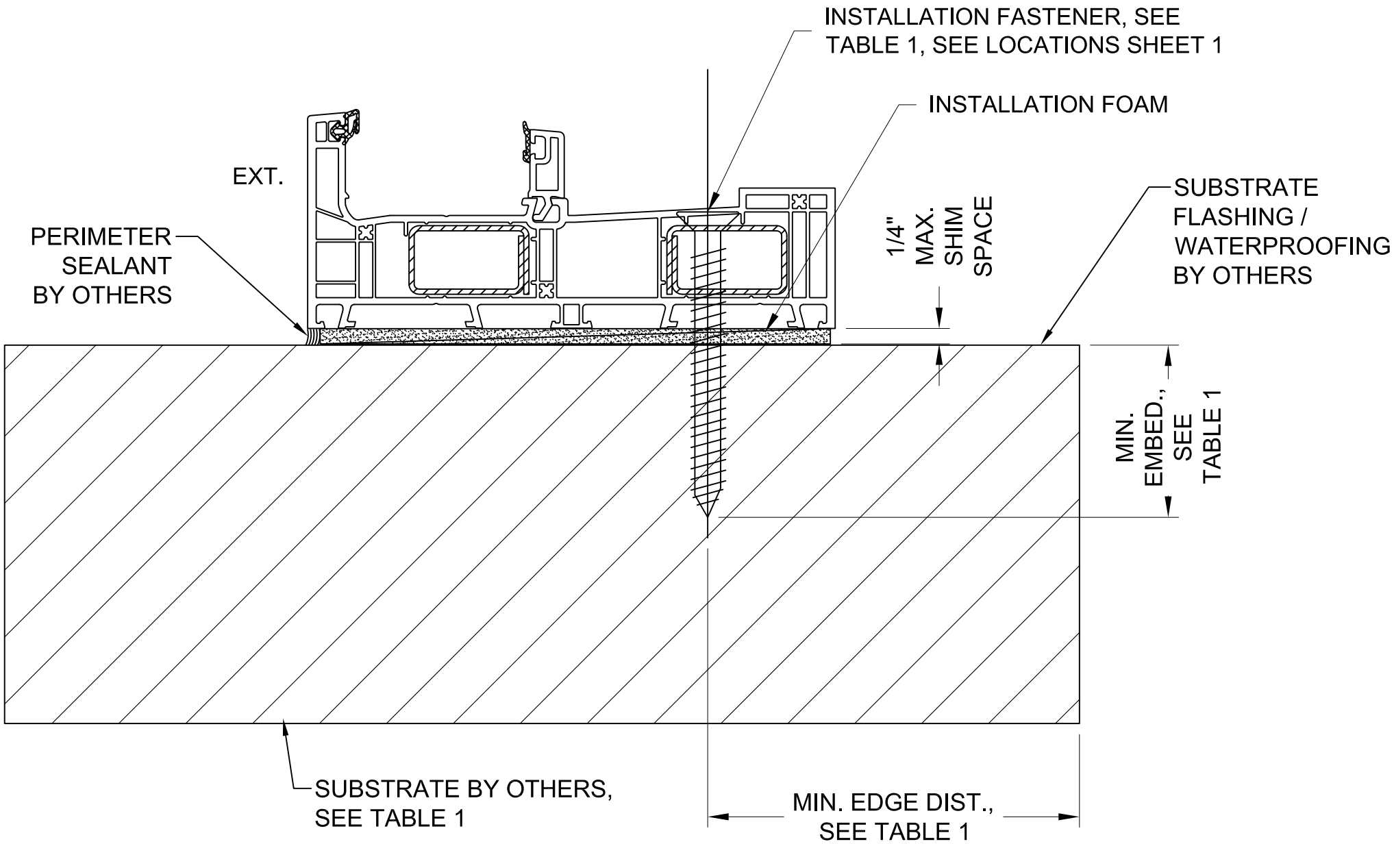
TYPICAL INSTALLATION, HEAD/SILL/JAMB
