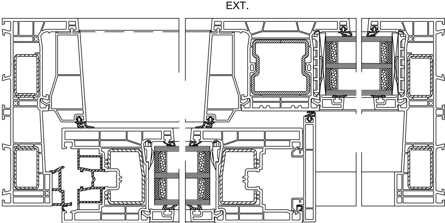
HORIZONTAL SECTION
