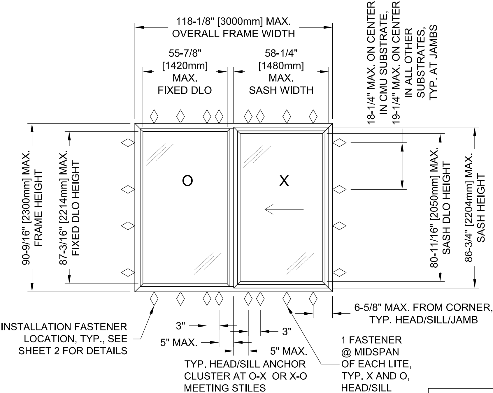
TYPICAL ELEVATION
