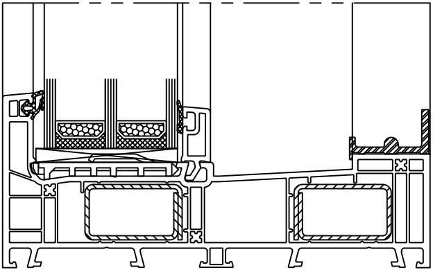
VERTICAL SECTION FIXED
