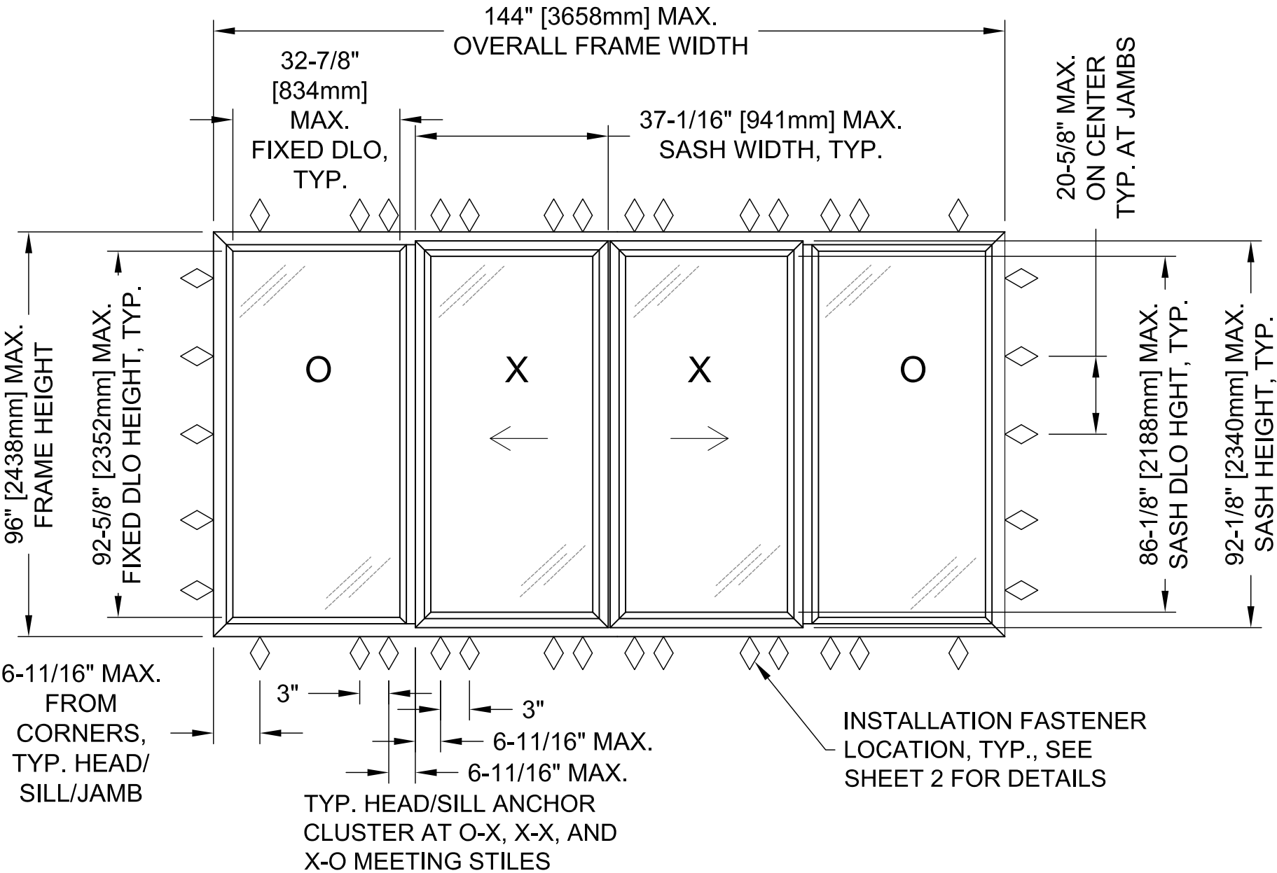
TYPICAL ELEVATION
