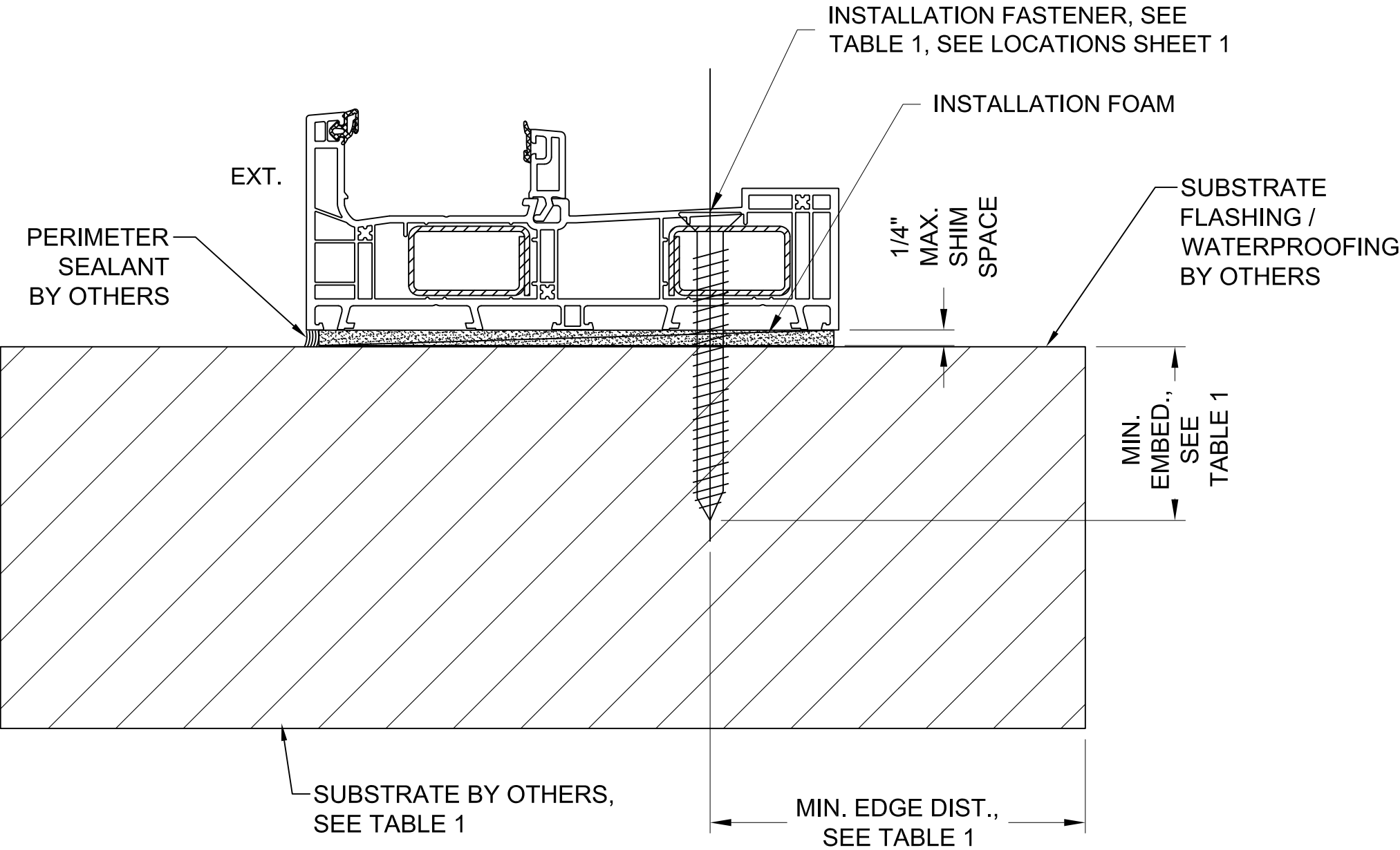
TYPICAL INSTALLATION, HEAD/SILL/JAMB
