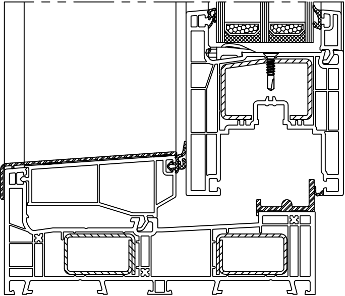
VERTICAL SECTION SASH
