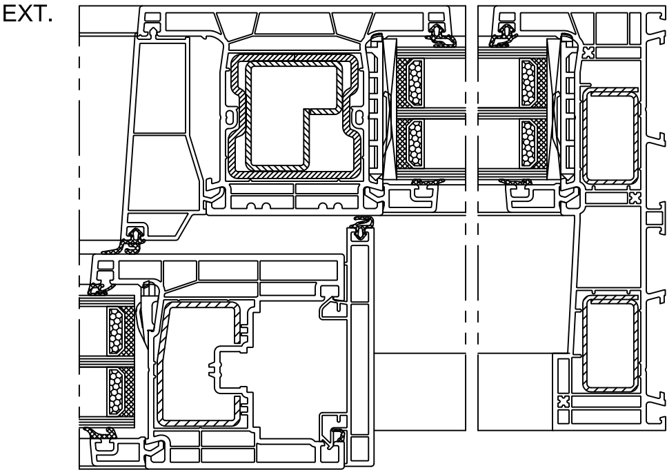
X-O AND JAMB HORIZONTAL SECTIONS
