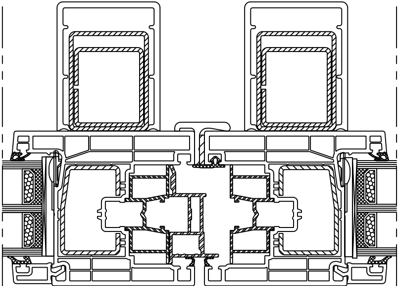
X-X HORIZONTAL SECTION
