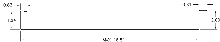
PANEL SECTION (24 GA.)
