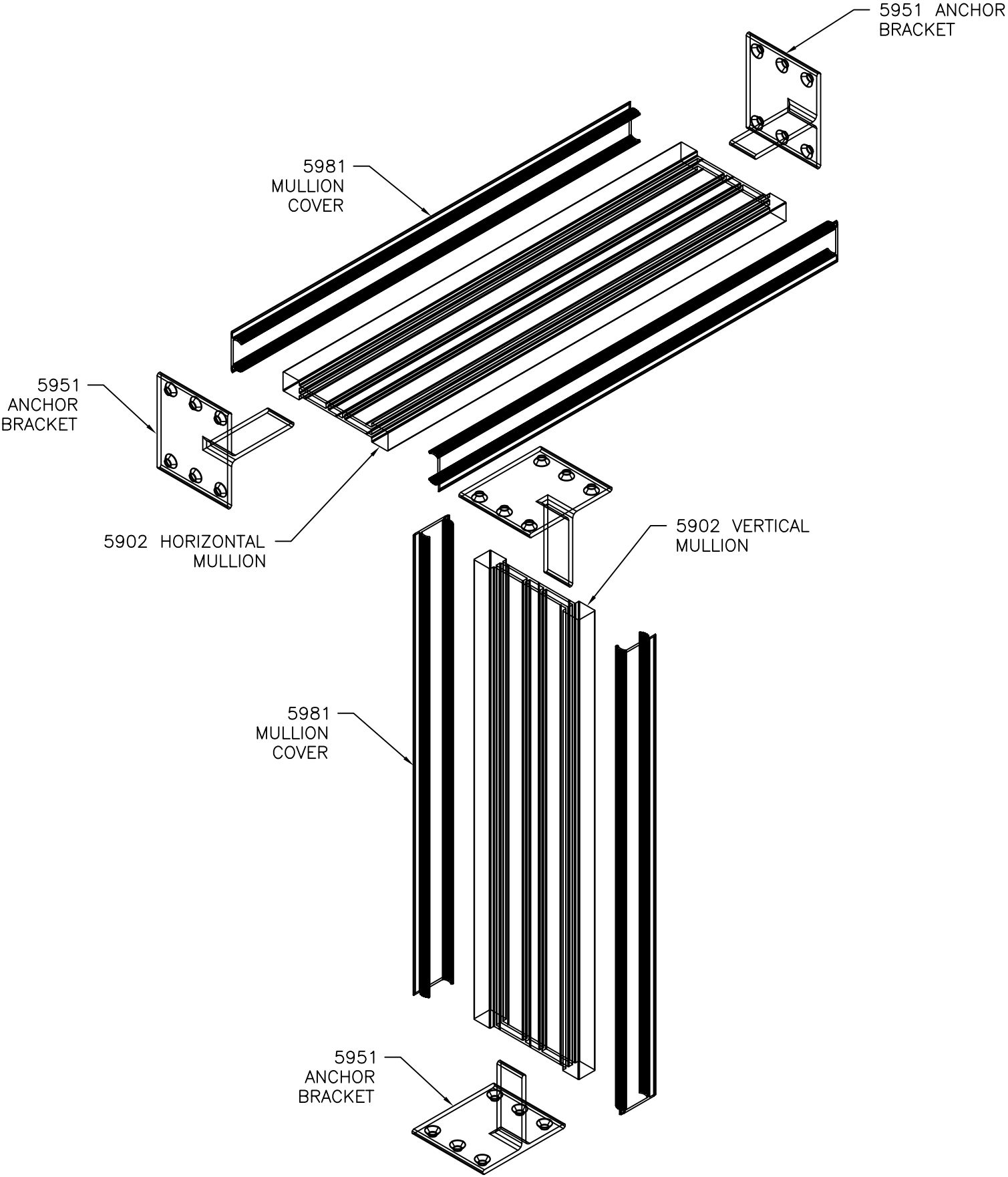
HORIZONTAL TO VERTICAL MULLION INSTALLATION
