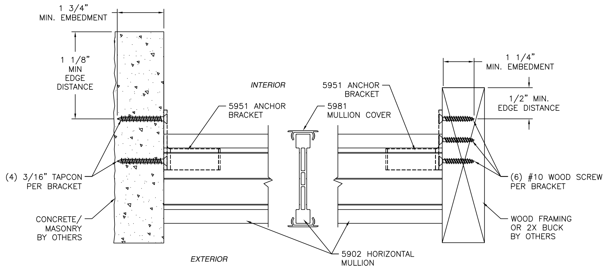
HORIZONTAL CROSS SECTION WOOD & CONCRETE INSTALLATION
