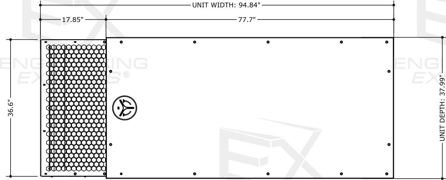
1 ENCLOSURE SIZE (A-GROUP) 3 NOT TO SCALE PLAN VIEW
