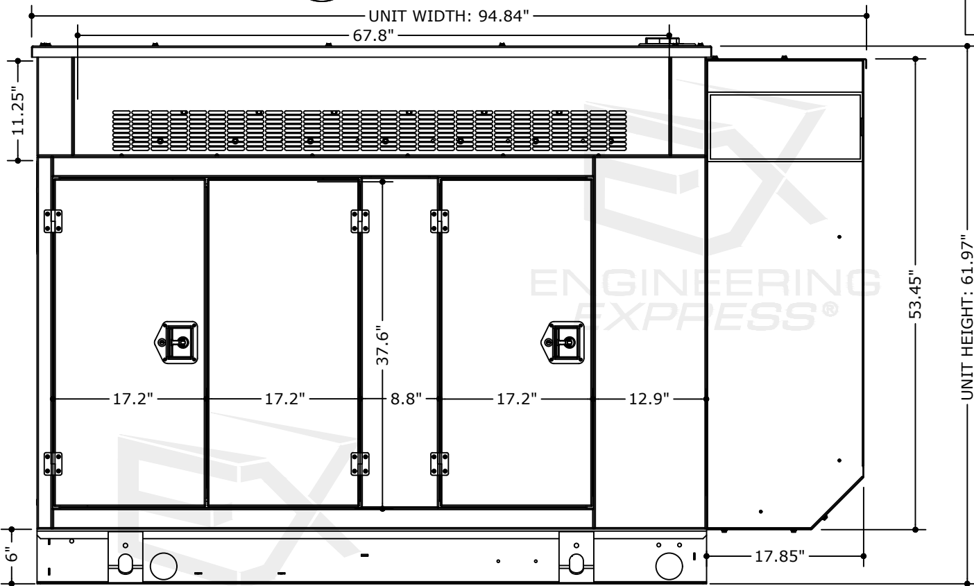
2 ENCLOSURE SIZE (A-GROUP) 2 NOT TO SCALE FRONT ELEV VIEW
