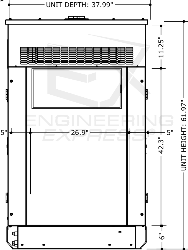
1 ENCLOSURE SIZE (A-GROUP) 2 NOT TO SCALE LEFT ELEV VIEW
