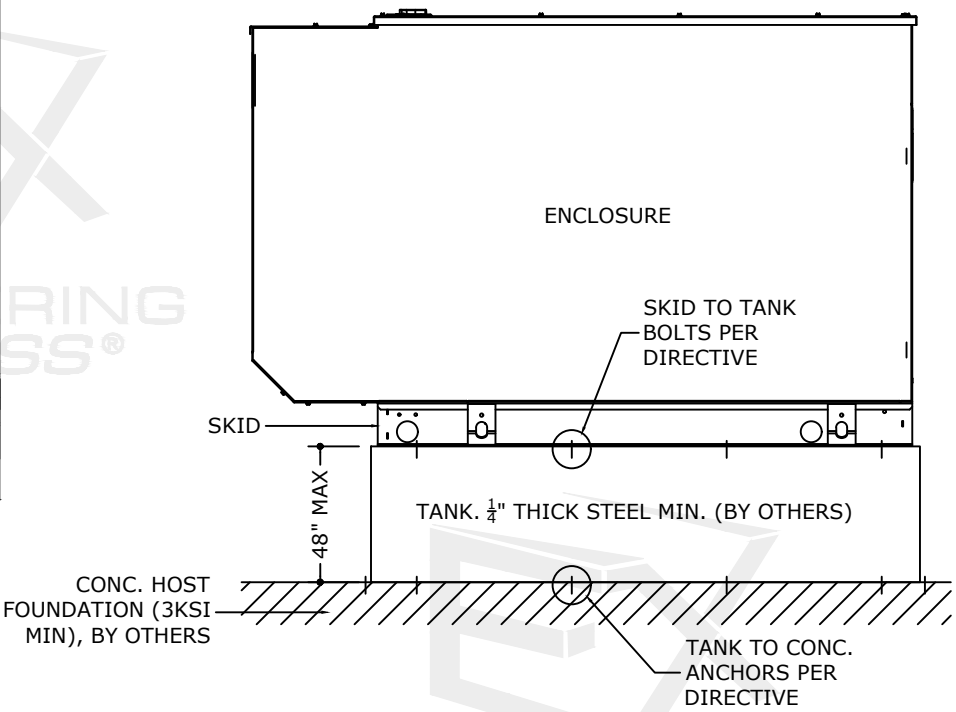
OPTION 2: ENCLOSURE TO TANK & TANK TO CONCRETE
