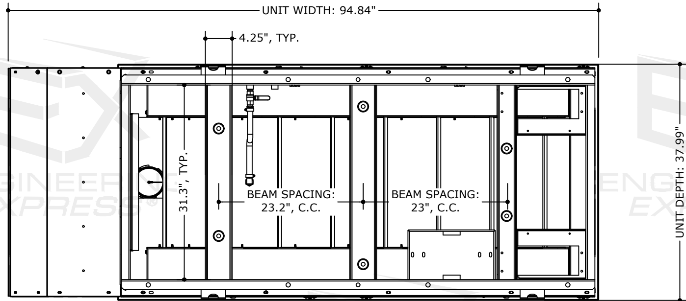
2 ENCLOSURE SIZE (A-GROUP) 3 NOT TO SCALE BOTTOM VIEW
