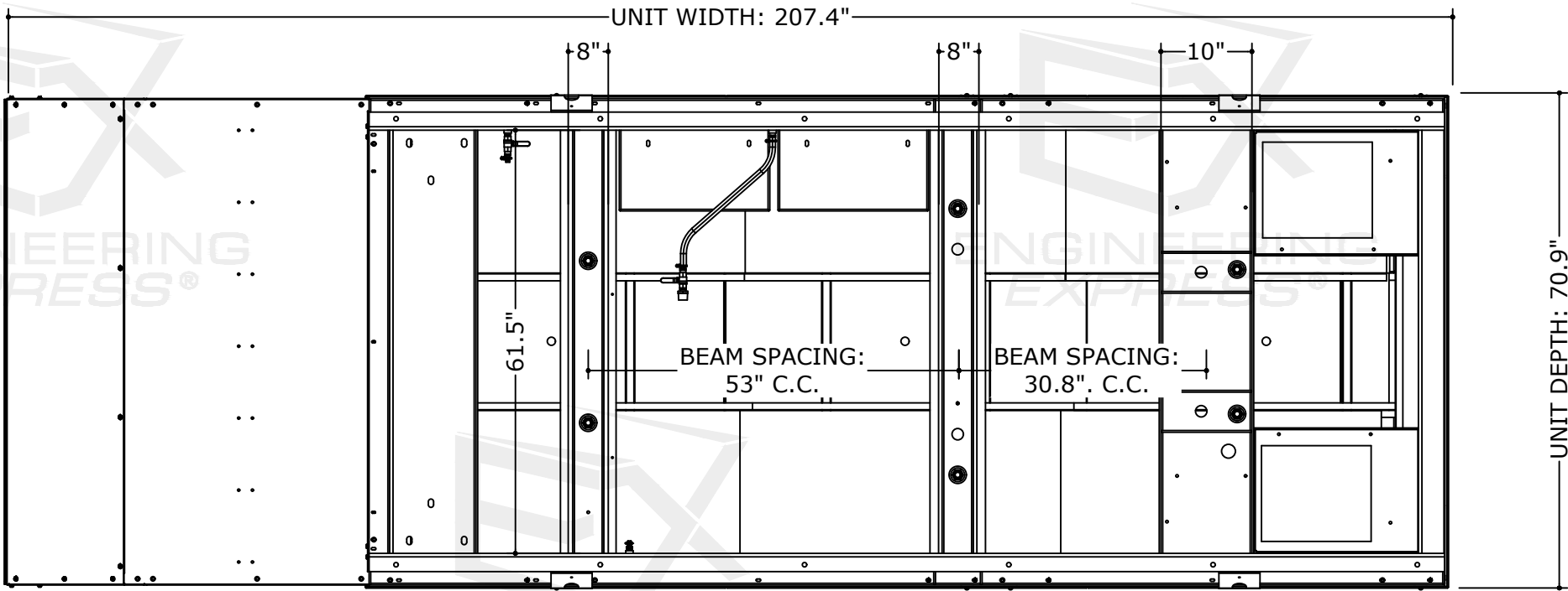
1 ENCLOSURE SIZE (H-GROUP) 10 NOT TO SCALE TOP VIEW
