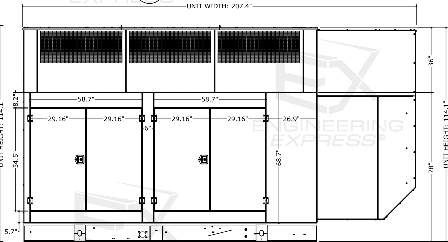
2 ENCLOSURE SIZE (H-GROUP) 9 NOT TO SCALE FRONT VIEW
