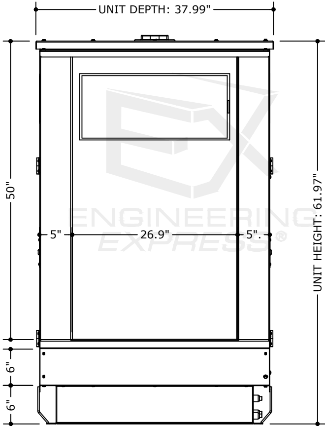
1 ENCLOSURE SIZE (A-GROUP) 2 NOT TO SCALE LEFT ELEV VIEW
