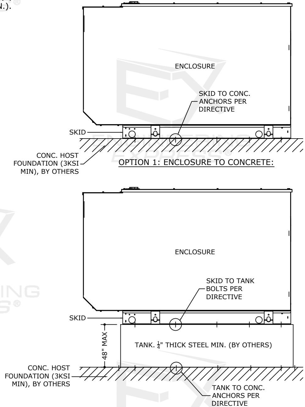
OPTION 2: ENCLOSURE TO TANK & TANK TO CONCRETE
