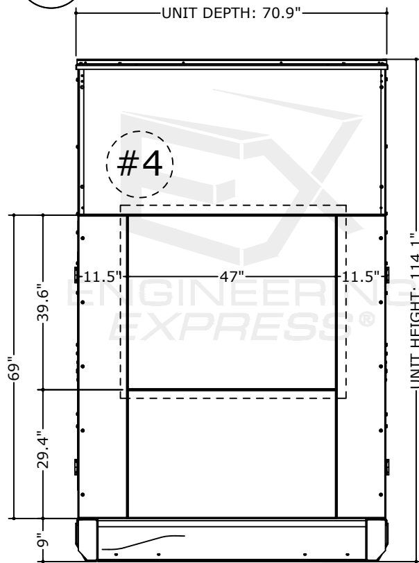
1 ENCLOSURE SIZE (H-GROUP) 9 NOT TO SCALE LEFT VIEW
