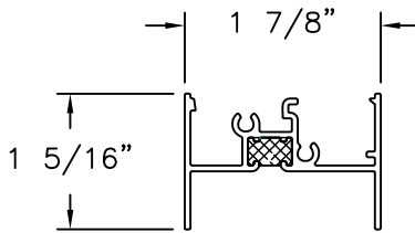
BI-FOLD HINGE ALUMINUM 6063-T6
