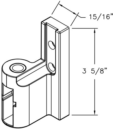
FLOATER KNUCKLE
